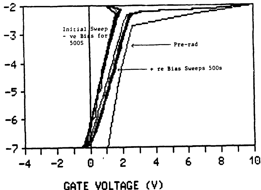
Figure 25: I-V response curves for 2N12 ( V_g = +10V , T = 100^\circ C ), with bias switching as described in text, following Flash X-ray irradiation.
