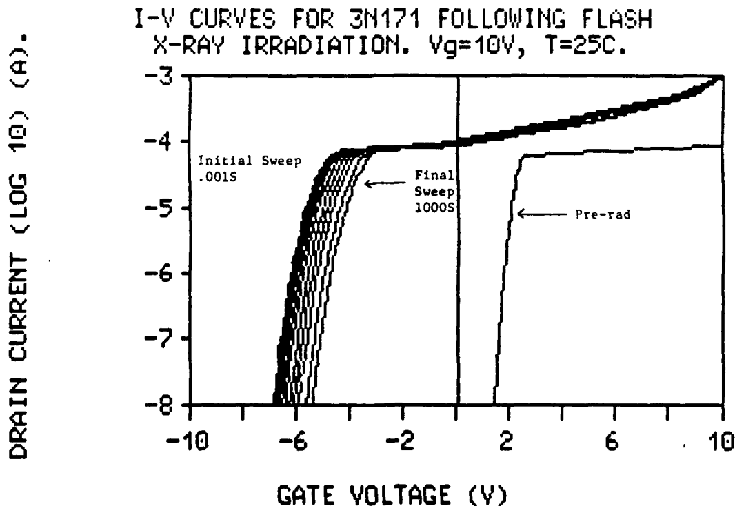
Figure 23: I-V response curves for 3N171 ( V_g = 10V , T = 25^\circ C ) following Flash X-ray irradiation. (Total dose \approx 10 kRad).
