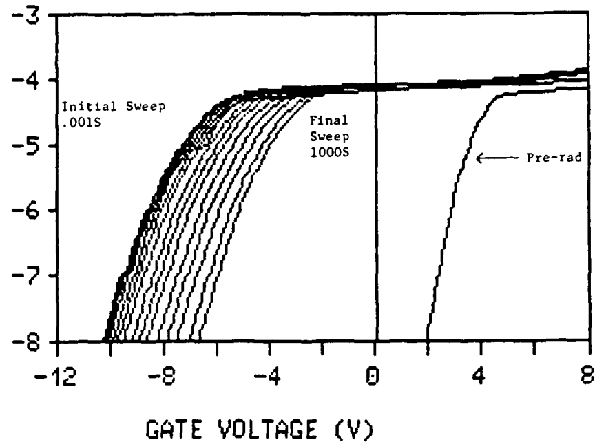
Figure 24: I-V response curve for 3N171 ( V_g = 20V , T = 100^\circ C ) following Flash X-ray irradiation. (Total dose \approx 10 kRad). The enhanced annealing compared to that in fig 23 is readily apparent.
