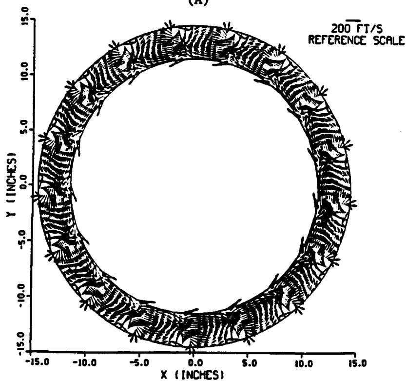
Figure 8. Rotor Velocity Distributions near Trailing Edge, \omega = 3550 rpm, Q = 16,000 cfm, (A) Axial (B) Radial and Tangential Components.
