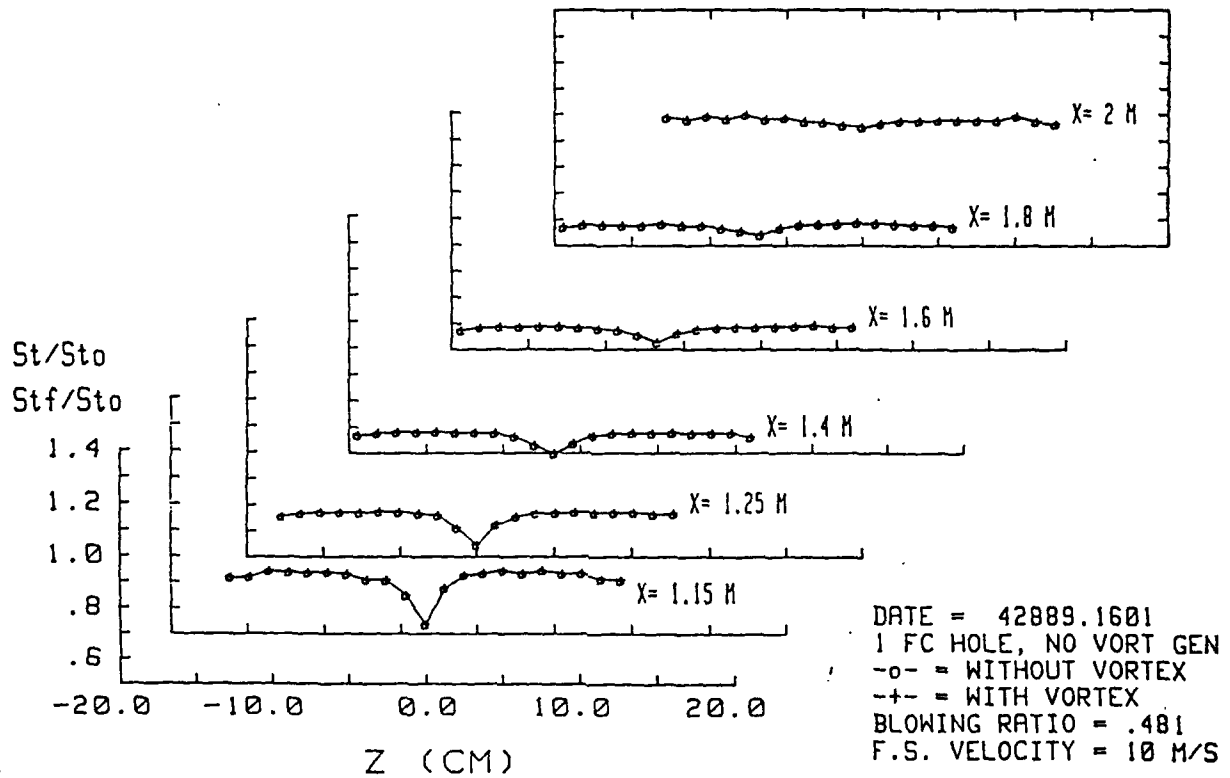
Figure 106 Local Stanton Number Ratios in Boundary Layers with Film-Cooling, with and without an embedded Vortex, A Single Injection Hole, m = 0.481 , No Vortex Generator
