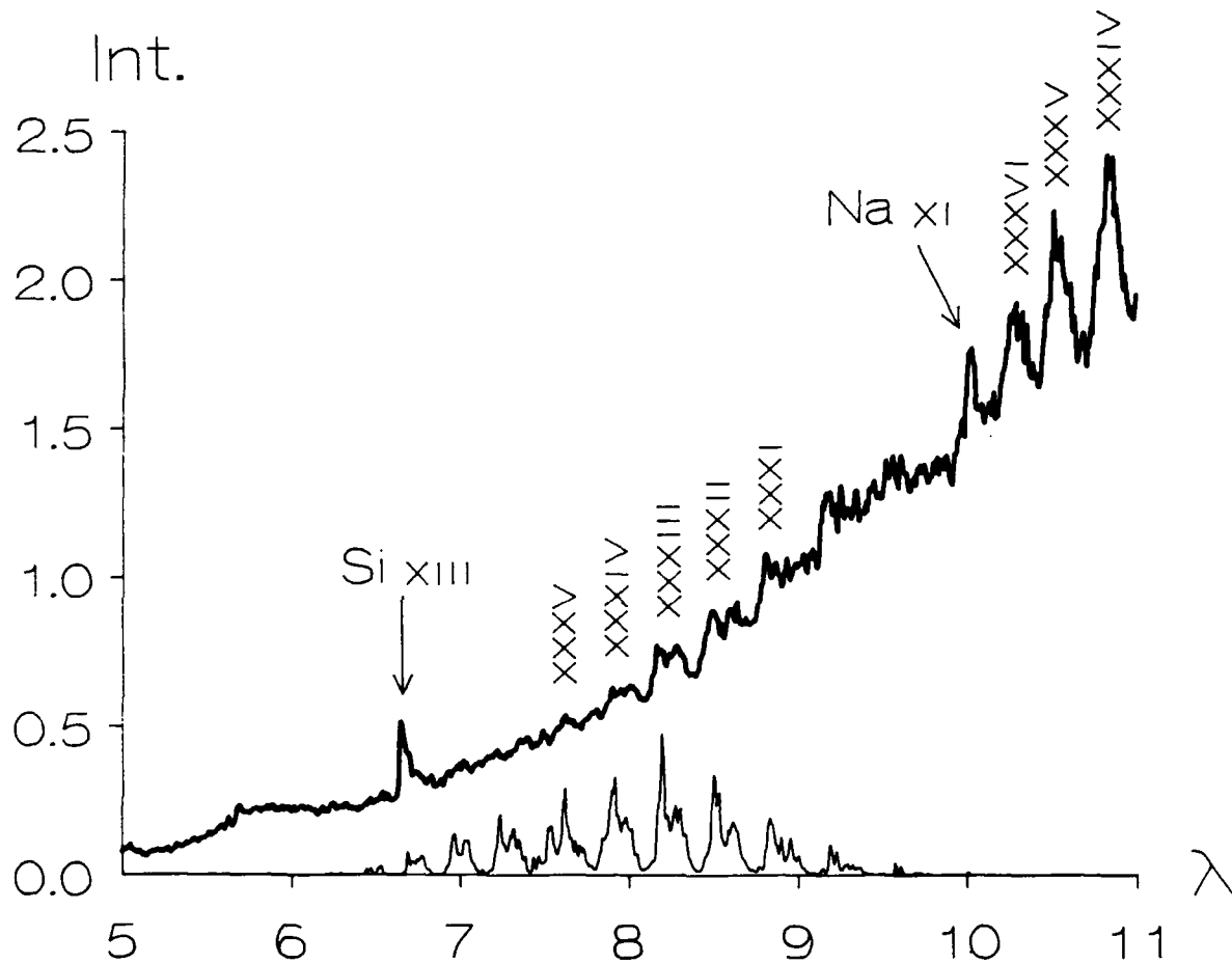
Fig. 5 — Experimental intensity trace from a laser-irradiated \text{BaBi}_{0.4}\text{Pb}_{0.6}\text{O}_3 compound (intensity in 10^{17} eV/sr-Å and wavelength in Å). The lower trace is a plot of the calculated gA values for the Ba ion transition sequence with 3d^{n-1}5f and 6f excited states.
