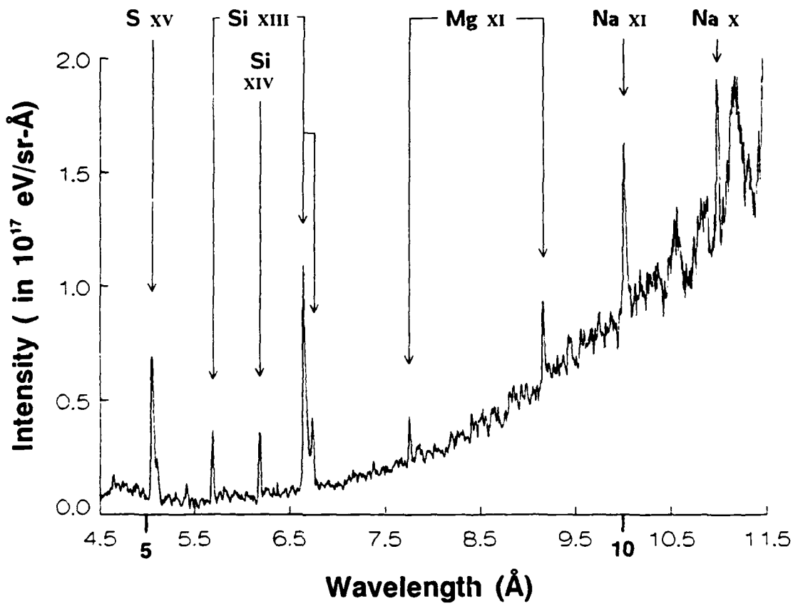
Fig. 3 — Spectral intensity trace from a BaBi 0.4 Pb 0.6 O 3 microfragment with impurity lines used for wavelength calibration
