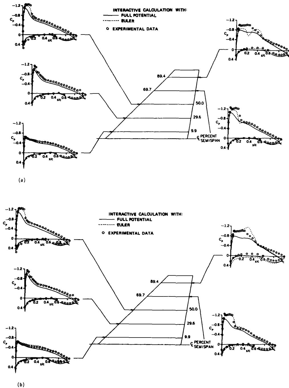
Figure 3. Comparison of calculated and experimental chordwise pressure distributions for M_\infty = 0.82 , Re = 6.8 \times 10^6 . (a) Euler with H-grid. (b) Euler with C-grid.
