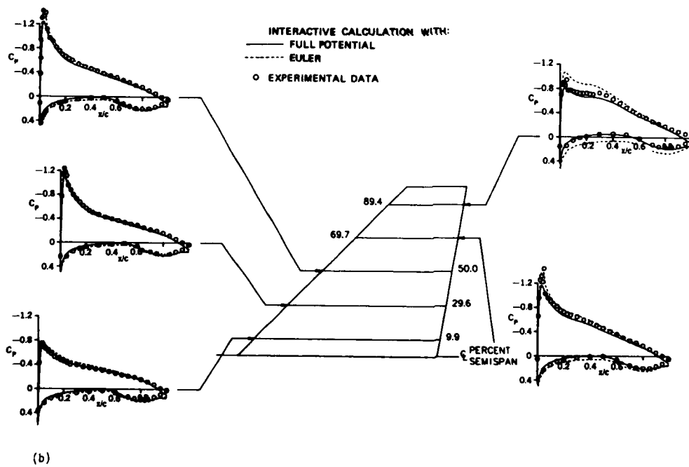
Figure 2. Comparison of calculated and experimental chordwise pressure distributions for M_\infty = 0.70 , Re = 6.8 \times 10^6 . (a) Euler with H-grid. (b) Euler with C-grid.
