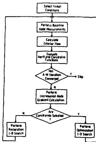
Figure 4. Automated Adaptive-Wall Iterative Procedure.
