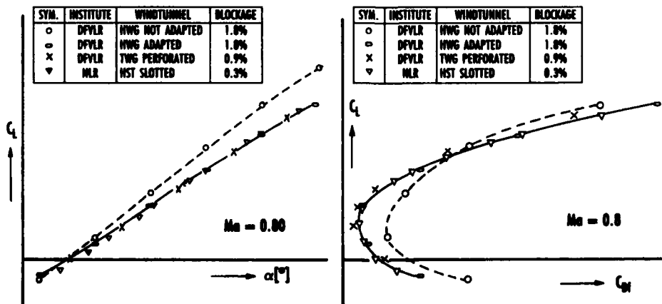
b. Lift coefficient vs angle-of-attack
