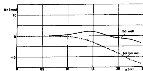
Fig. 4.12: Typical wall displacement for lift model.
