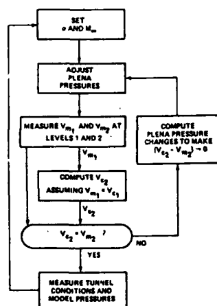
Fig. 2 Adaptive-wall wind-tunnel scheme.
