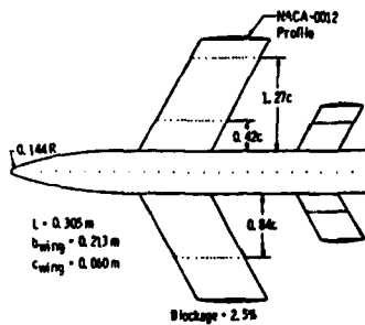
Figure 3. Generic Wall Interference Model.
