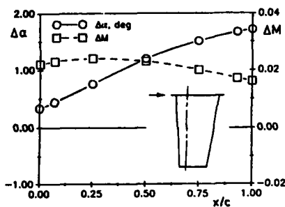
Fig. 4.16: Chordwise variation of wall interference; walls straight, M_\infty = 0.7 , \alpha = 7^\circ , wing high
