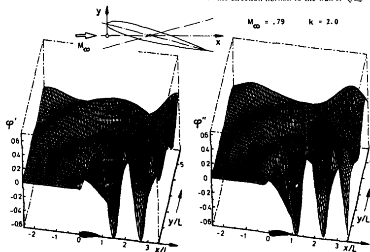
Fig.7.2: Motion-induced unsteady flow field (complex unsteady potential function \phi ) of an airfoil performing harmonic pitching oscillations about the 0.425-chord axis ( \phi' = real part, \phi'' = imaginary part of \phi )
