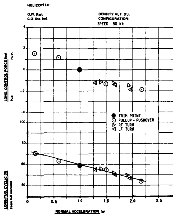
Figure 1.27 - MANOEUVRING STABILITY
