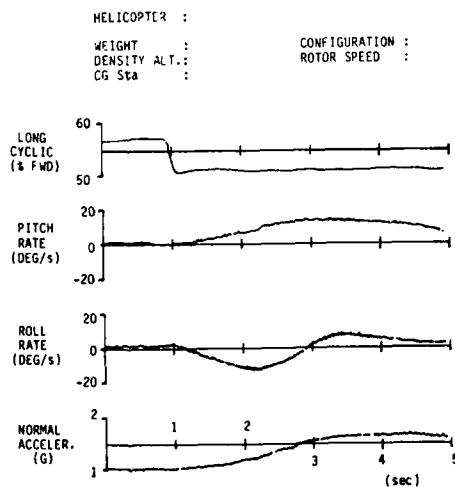
Figure 1.21 - CONTROL RESPONSE LONG. RWD 80 Kt
