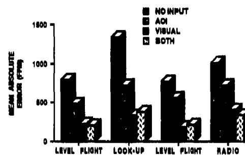
Figure 5. Deviation of vertical velocity from zero fpm
