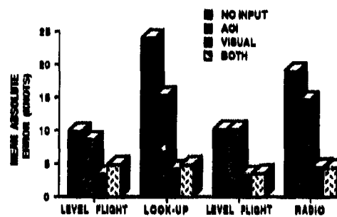
Figure 6. Deviation of airspeed from 300 knots
