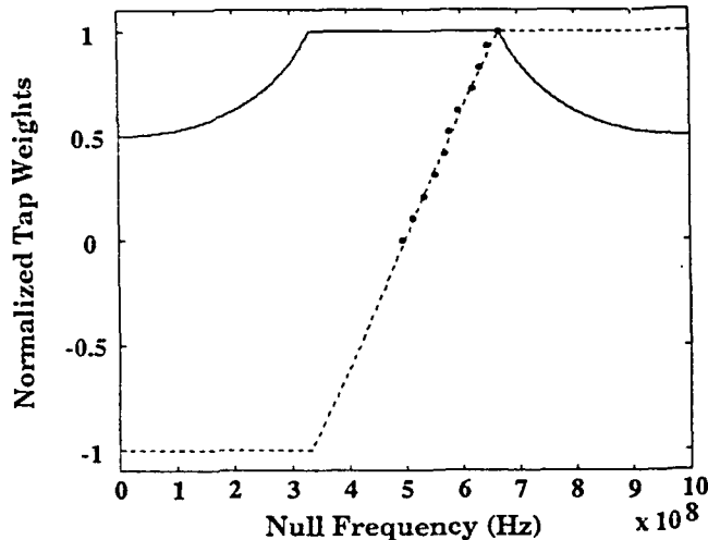
Fig. 3. Demonstration of null frequency shifting by varying center tap weight (dotted curve) with first and third tap weight held constant (solid curve).
