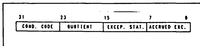
Figure 38 FPCR Status Register
