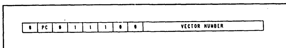
Figure 59 Take Pre-instruction Exception format
