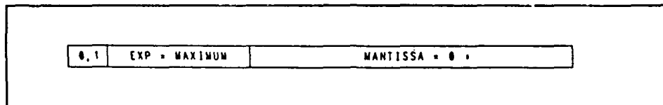
Figure 50 Infinity format
