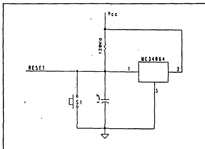
Figure 65 Reset Circuit
