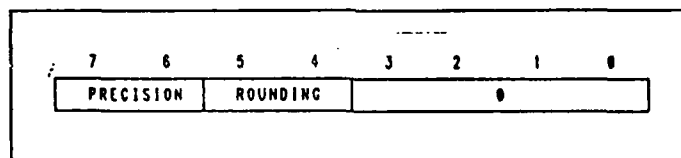
Figure 37 FPCR Mode Control byte
