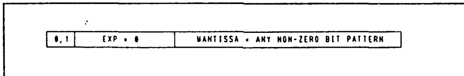
Figure 48 Denormalized Number Format
