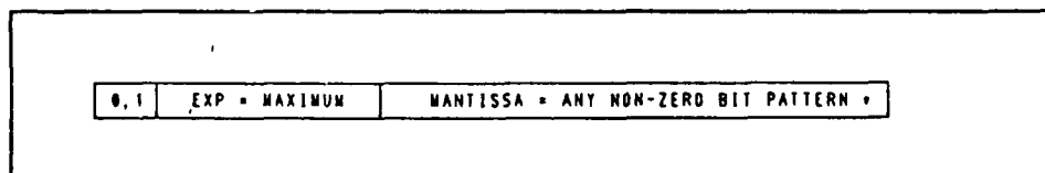
Figure 51 Not-A-Number format
