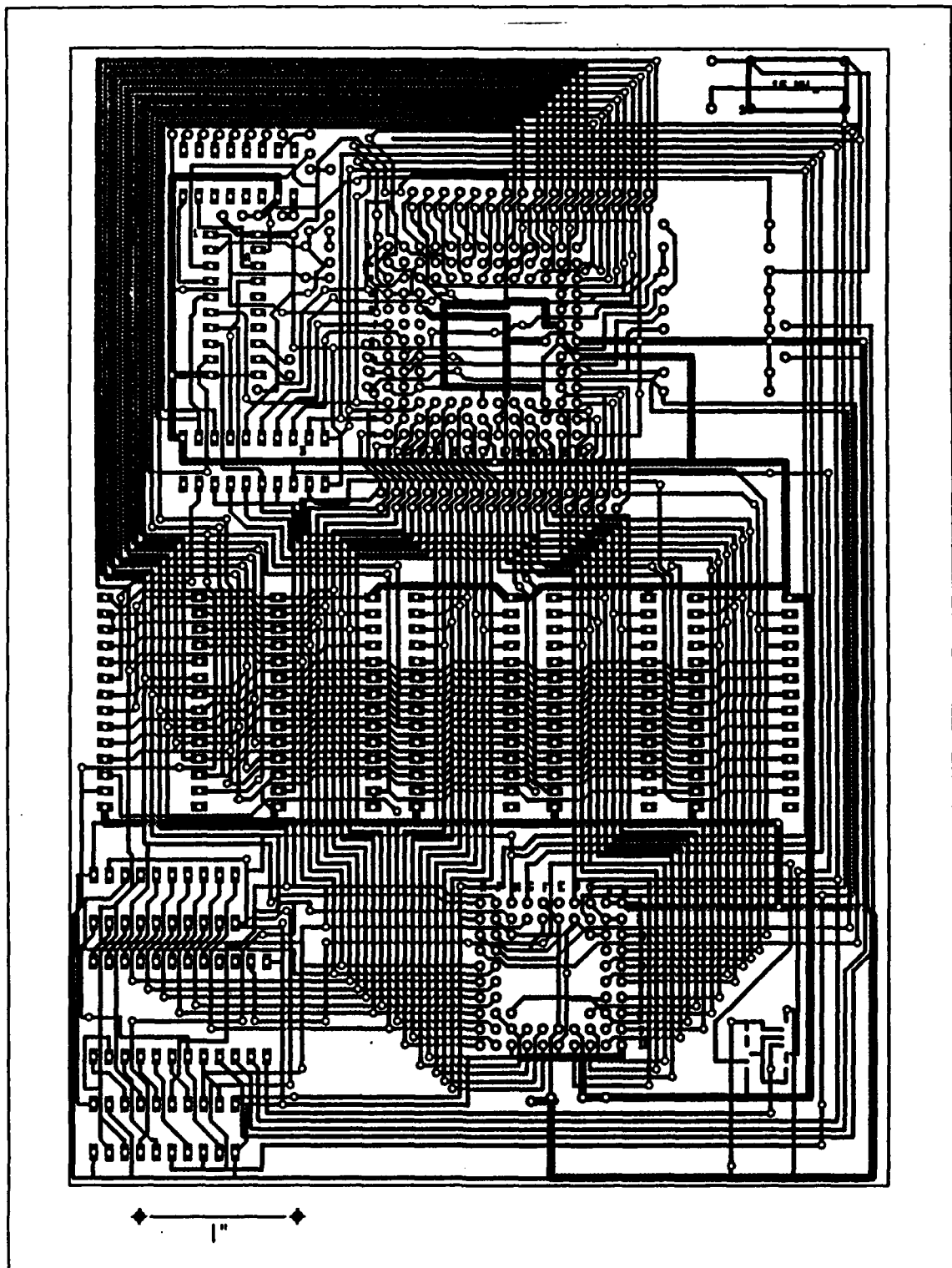
Figure 69 ECB Two Layer PCB Layout
