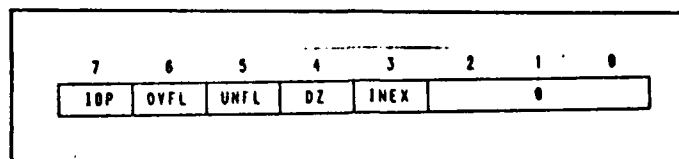
Figure 42 FPSR Accrued Exception byte
