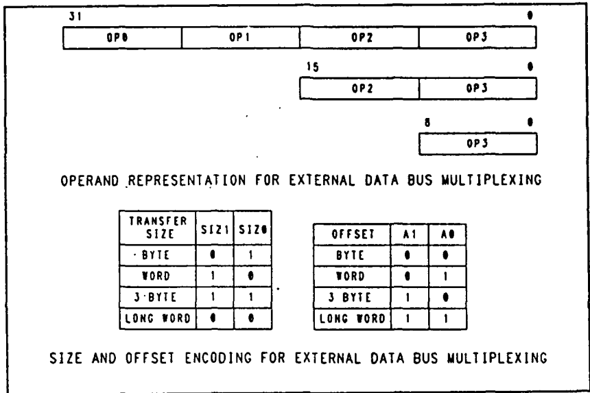
Figure 24 Operand representation and size/offset encodings
