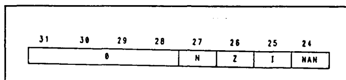
Figure 39 FPSR Condition Code byte
