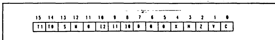
Figure 1 Status Register
