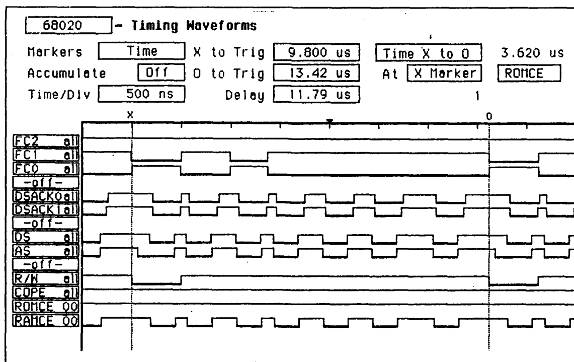
Figure 10 Timing diagram for RAM read/write test.
