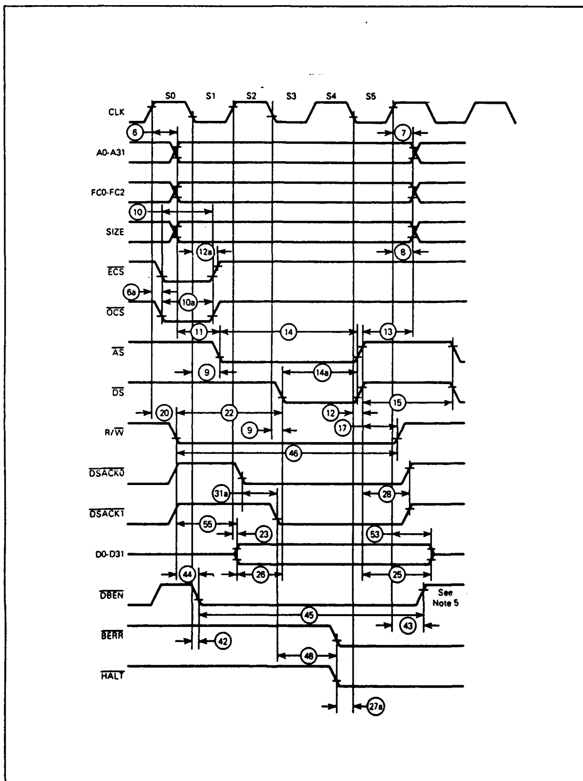
Figure 21 MC68020 Write Cycle Timing Diagram. (Copied from Reference 2)
