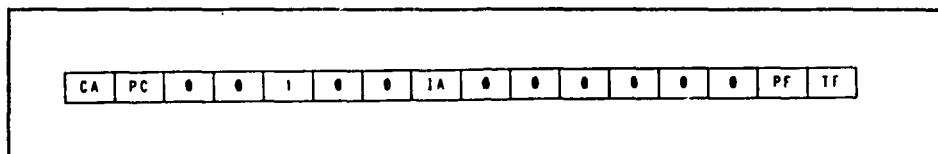
Figure 55 Null Format
