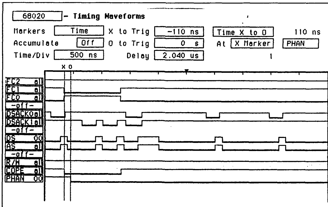
Figure 7 Timing waveforms for CopE and Phantom signals.
