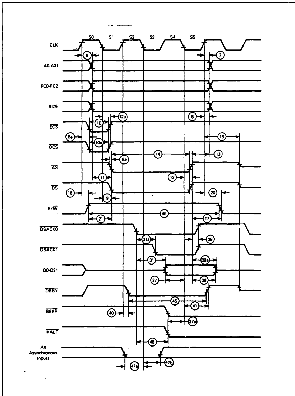
Figure 20 MC68020 Read Cycle Timing Diagram. (Copied from Reference 2)
