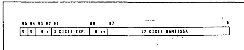
Figure 46 Packed Decimal Real data format
