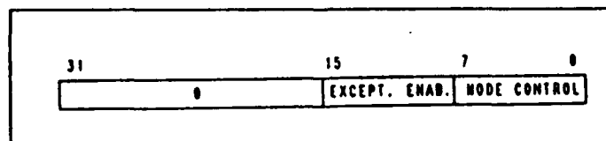
Figure 35 Floating Point Control Register
