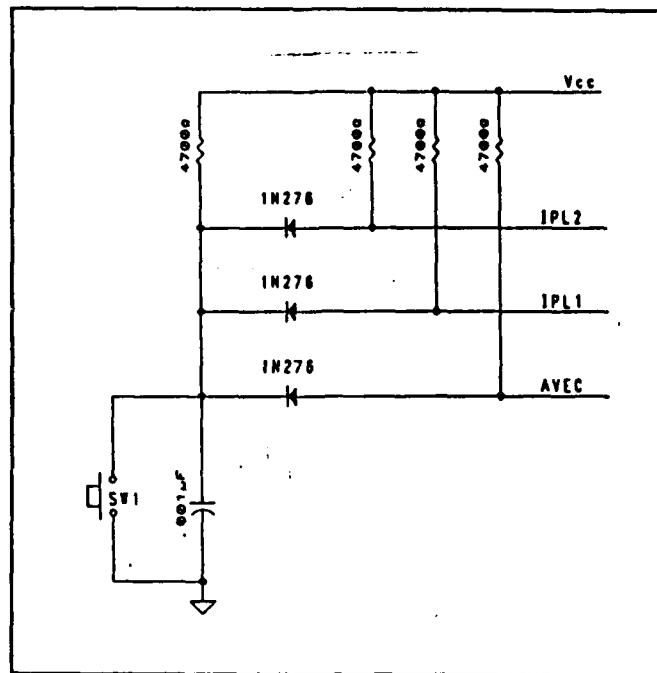
Figure 66 Software Abort circuit
