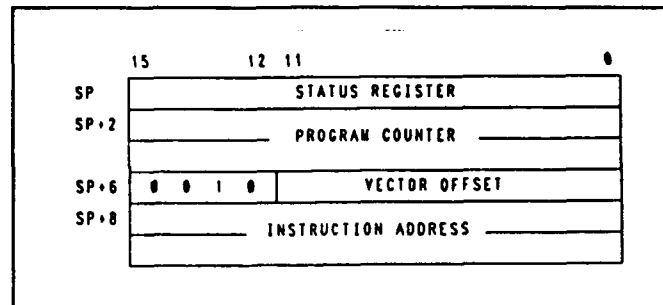
Figure 31 Normal six-word stack frame
