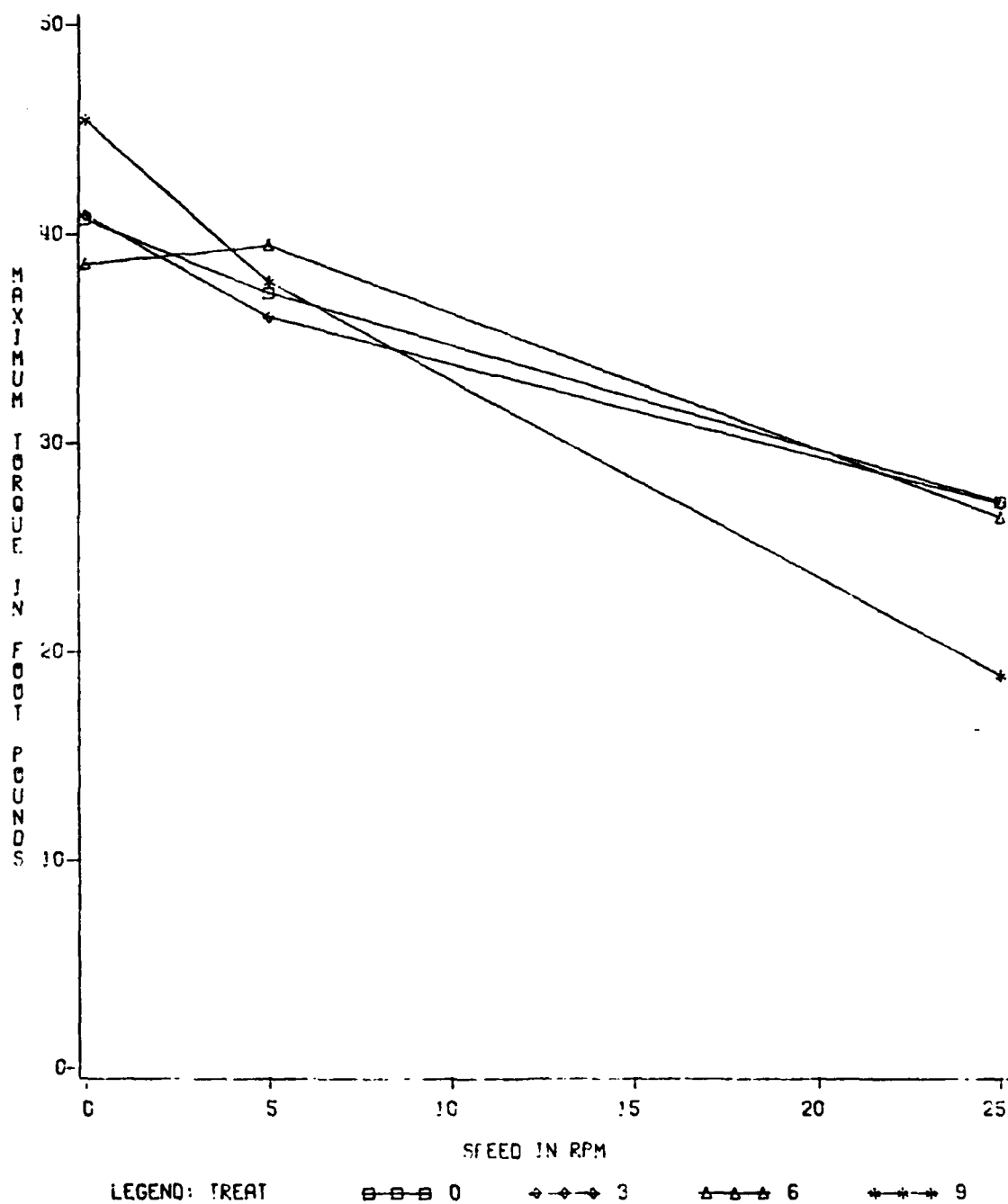
FIGURE 53 MAXIMUM TORQUE VS SPEED FOR VFE AND ROTATION OF 15 DEGREES
