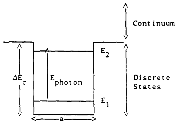
Figure 2 an energy level diagram for a finite depth quantum well showing the dominant intersubband transition and the energy regimes where discrete states and continuum states can be found.
