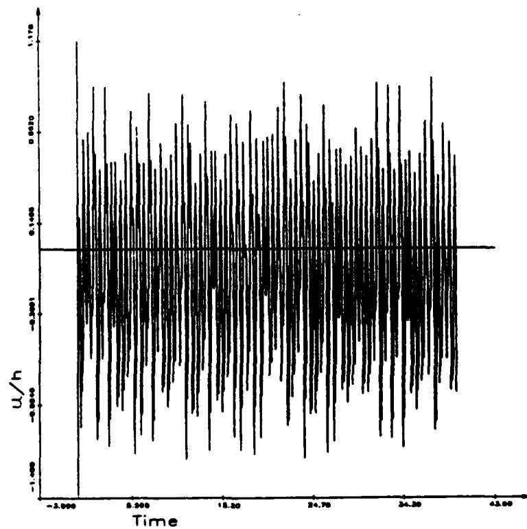
Figure 12(b) Chaotic response for \lambda = 150 , R_s = -3.0\pi^2 , and n = 1.28
