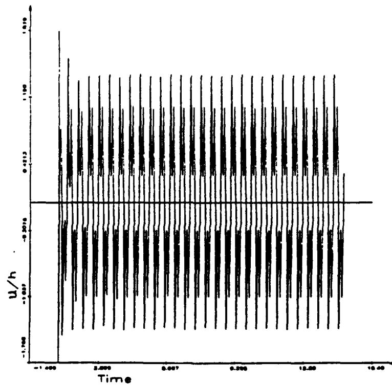
Figure 11(b) Phase plane response a_1 = 0.251 (period 1 motion)
