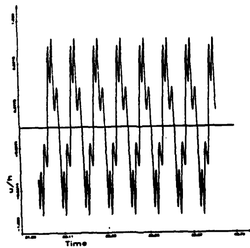
Figure 10 New more complicated limit cycle response for \lambda = 119.5 , and R_\infty = -4.0\pi^2
