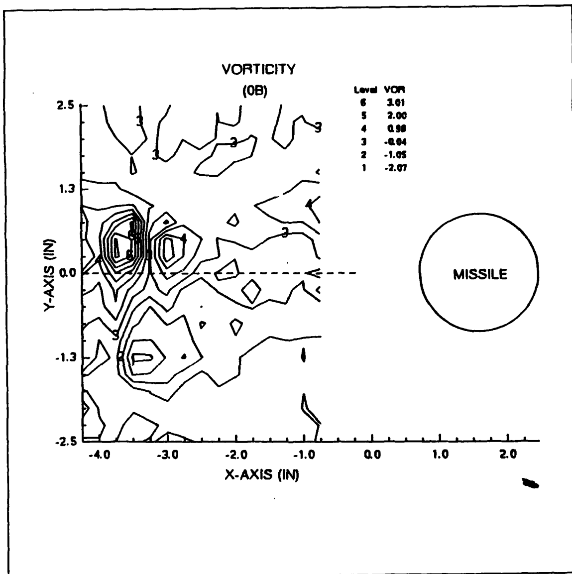
Figure 14. Vorticity-Configuration 0B
