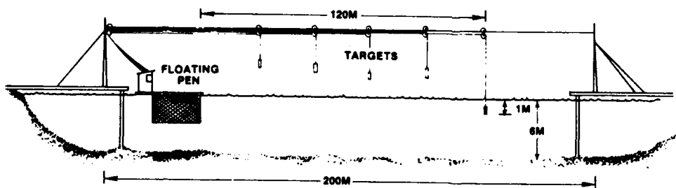
FIG. 1. Target range (Skyhook II) located in Kaneohe Bay, Oahu, Hawaii.
