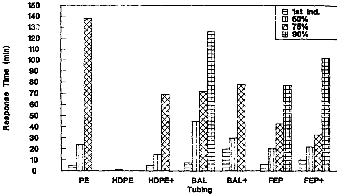
Figure 20. Response times of 61 m (200 ft) of tubing to 100 ppb hydrazine
