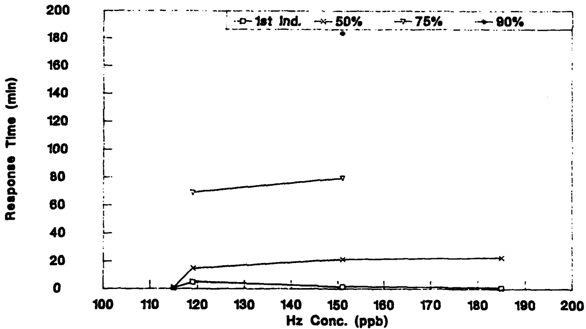
Figure 23. Effect of hydrazine concentration on 61 m (200 ft) of high density polyethylene tubing response time
