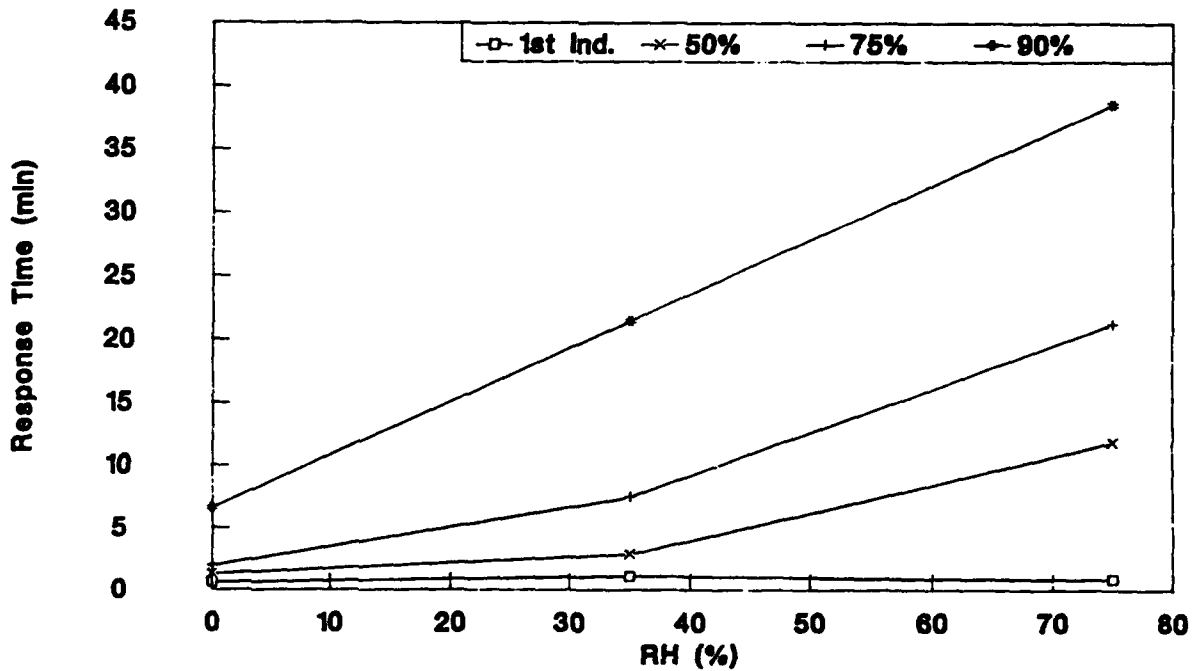
Figure 15. Relative humidity effects on 61 m (200 ft) of FEP exposed to TLV UDMH
