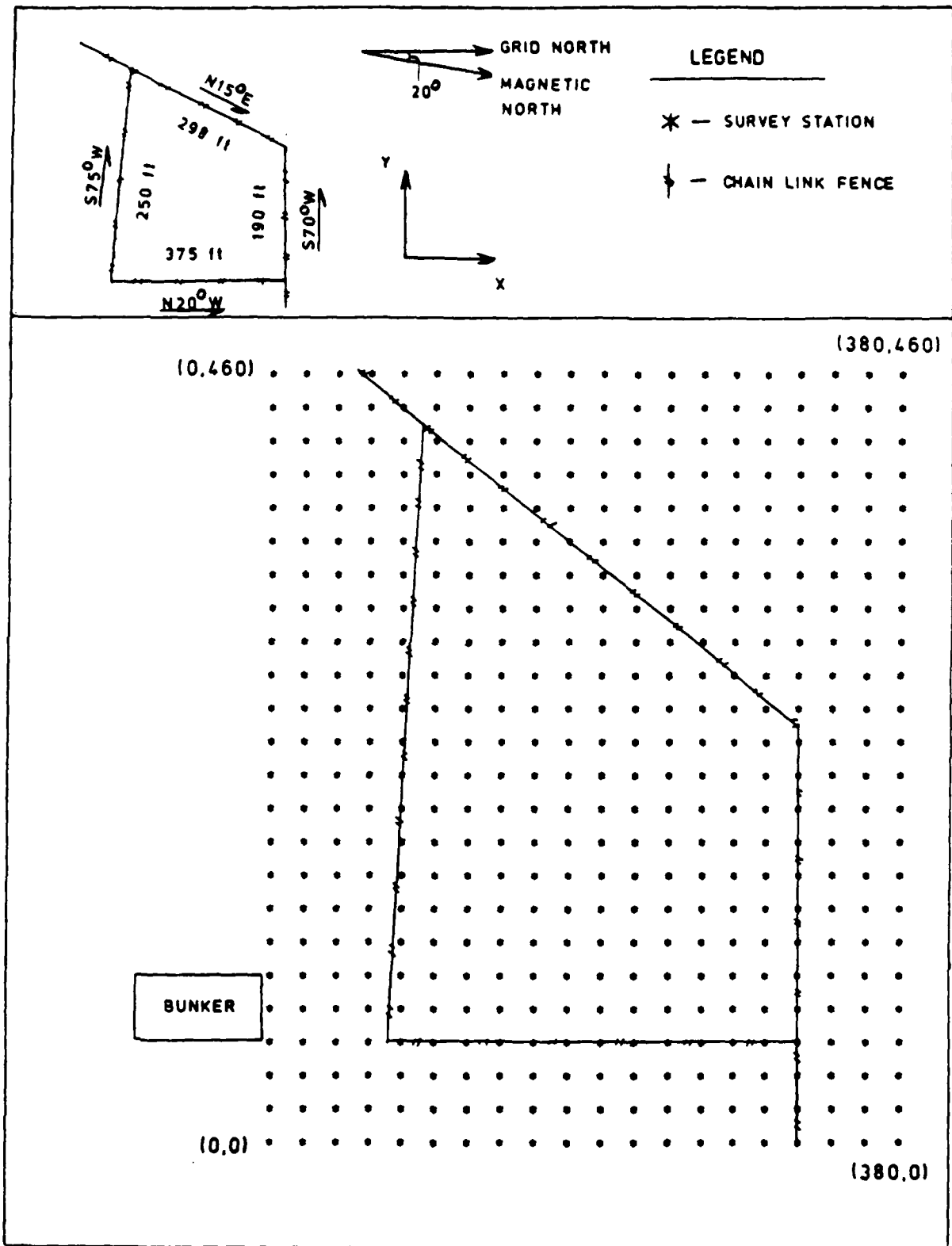
Figure 4. Grid layout for geophysical work conducted at the 3-A burial site.
