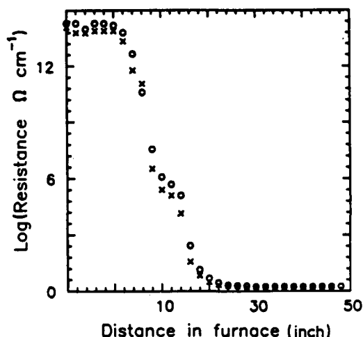
Figure 6 Change in electrical resistance during carbonization of precursor III. (○) 1 ft min -1 , (×) 6 inch min -1 .
