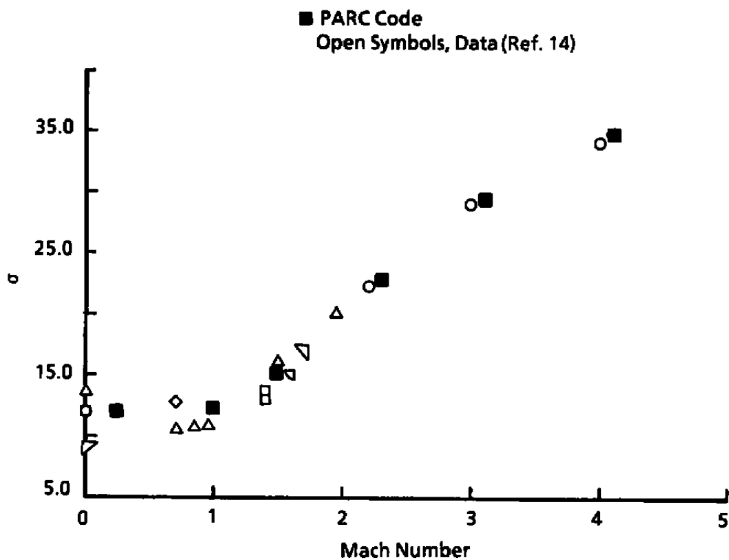
Figure 29. Supersonic jet spread rate comparison.
