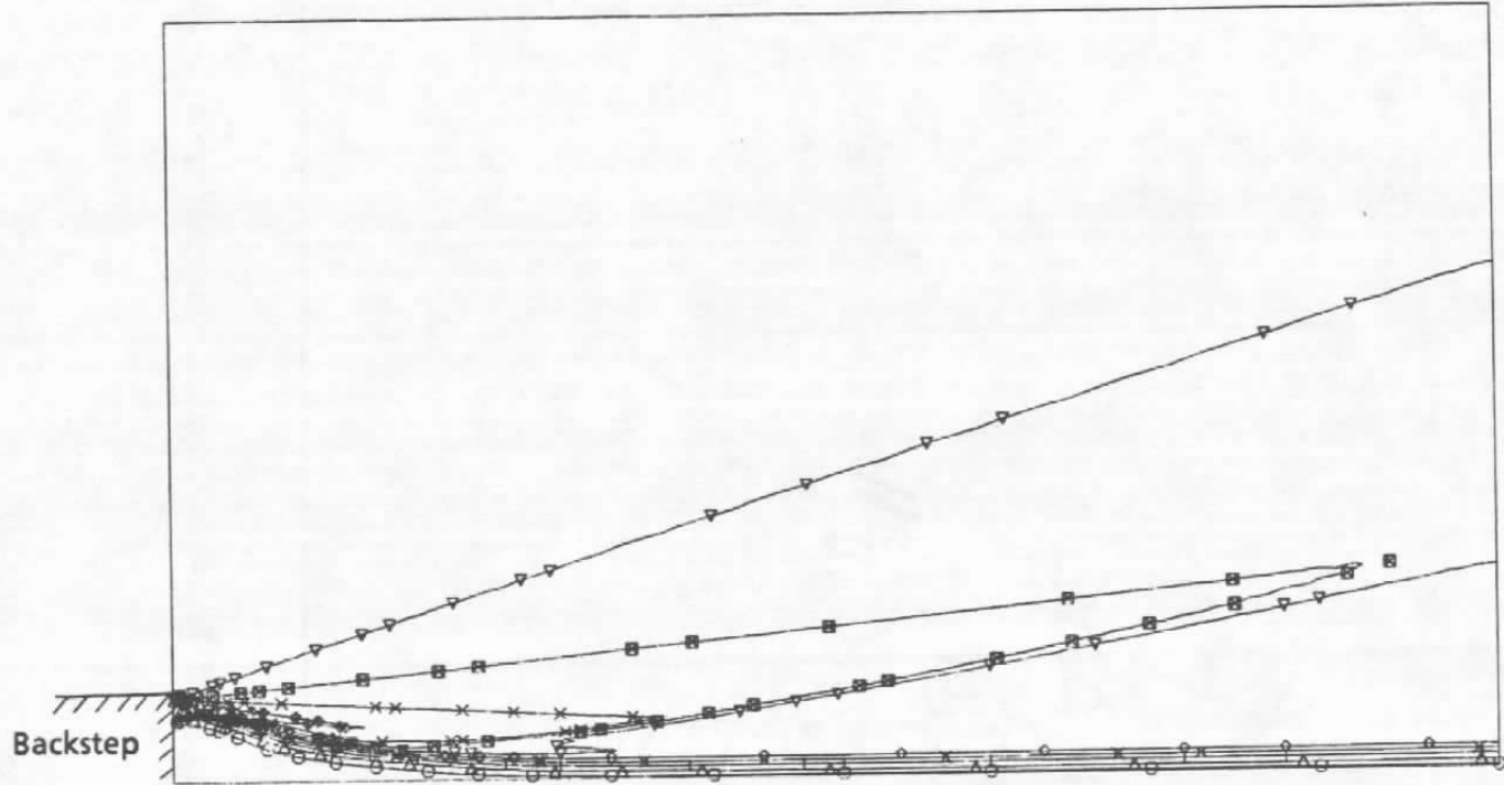
Figure 58. Rearward-facing step Mach 3.5 flow solution.
