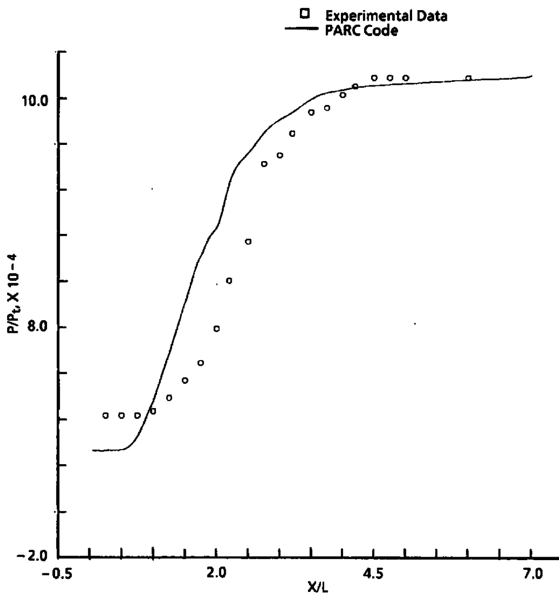
Figure 61. Rearward-facing step Mach 5.0 wall static pressure comparison.
