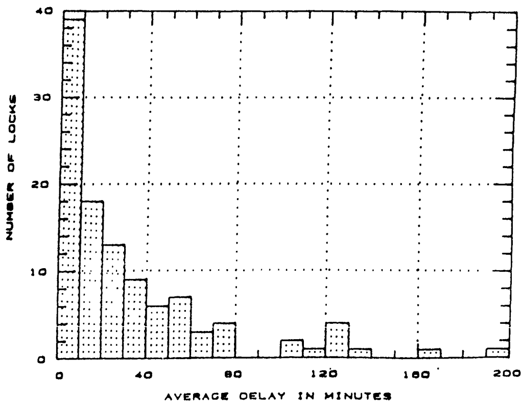
FIGURE 3.9 DISTRIBUTION OF AVERAGE DELAY TIME LOCKS < 200 MINUTES AVERAGE DELAY 1967
