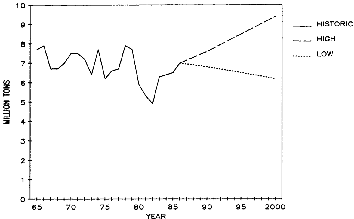
FIGURE 2.4 SEGMENT NUMBER 2 MISSOURI RIVER TRAFFIC HISTORIC 1965-1986 AND PROJECTED 1990, 1995 AND 2000
