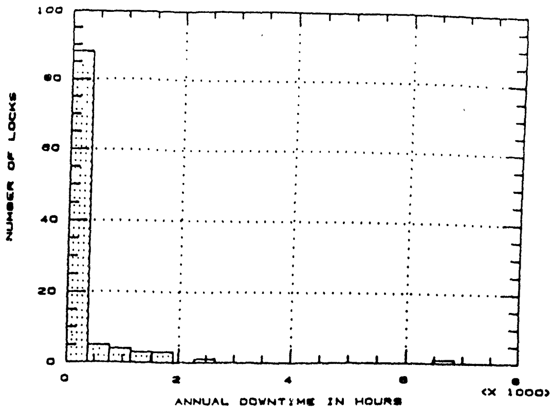
FIGURE 3.14 DISTRIBUTION OF ANNUAL DOWNTIME SELECTED LOCKS 1987
