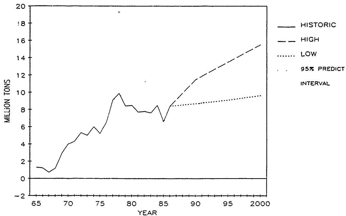
FIGURE A-3-3B SEGMENT NUMBER 3 ARKANSAS RIVER TRAFFIC HISTORIC 1965-1986 AND PROJECTED 1990, 1995 AND 2000
