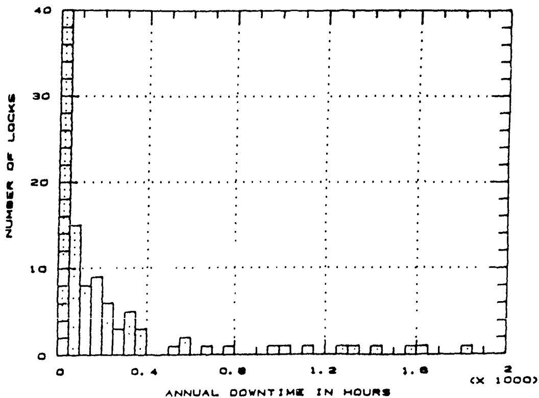
FIGURE 3.15 DISTRIBUTION OF ANNUAL DOWNTIME LOCKS < 2000 HOURS DOWNTIME 1987
