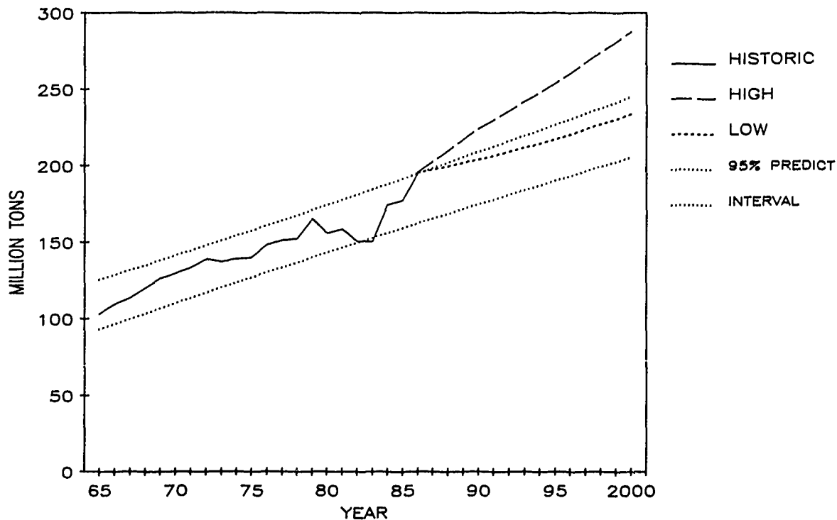
FIGURE 2.9 SEGMENT NUMBER 5 OHIO RIVER-MAINSTEM TRAFFIC HISTORIC 1965-1986 AND PROJECTED 1990, 1995 AND 2000
