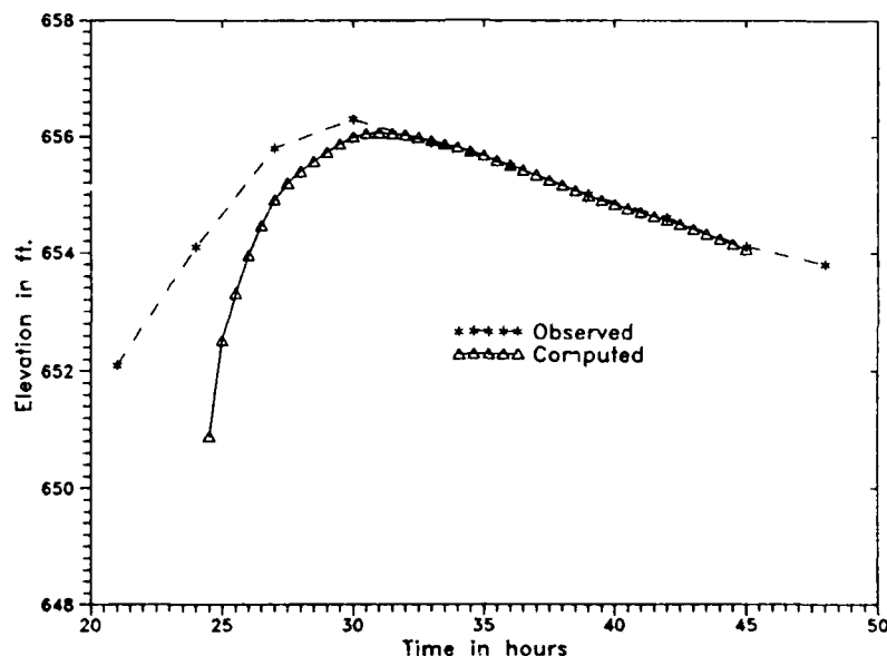
Figure 3. Upstream Stages, n_{ob} = 0.070
