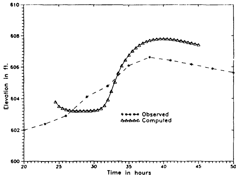
Figure 4. Downstream Stages, n_{ob} = 0.070
