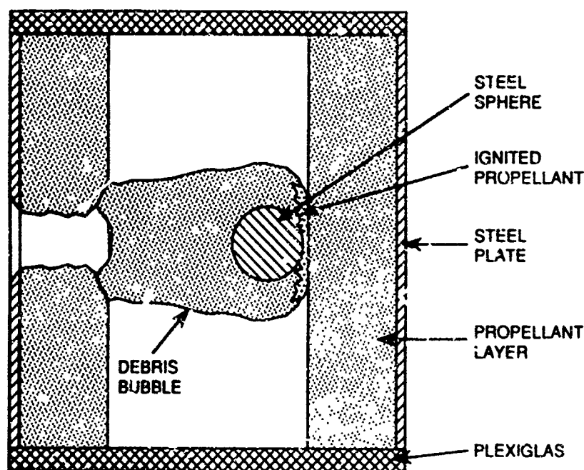
FIGURE 5. Sketch of Debris Bubble Ignition Process.
