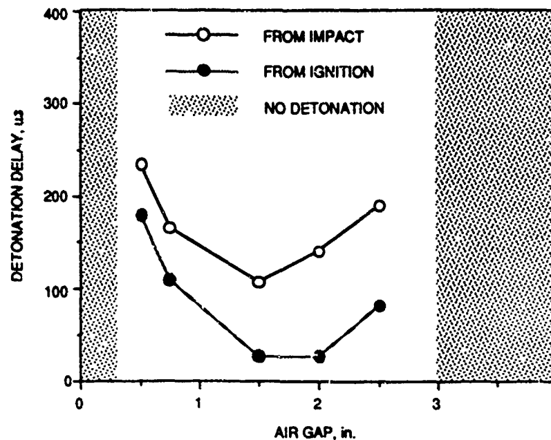
FIGURE 8. Detonation Delay Times for HEP-2 Propellant (Tests 16 Through 22).
