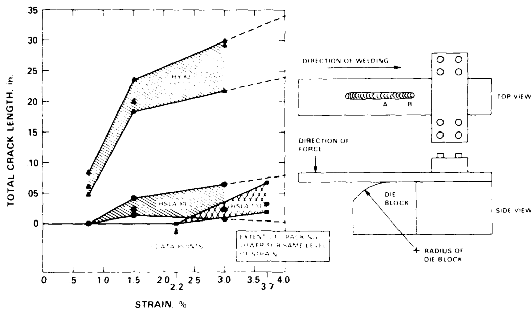
Fig. 7. Results of varestraint tests of high strength steels for hot cracking resistance.
