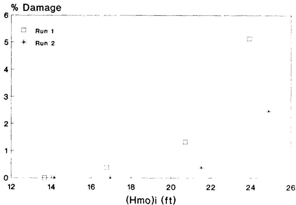
Figure 11. Harbor-side damage, Plan 2, "A-1" Stone
