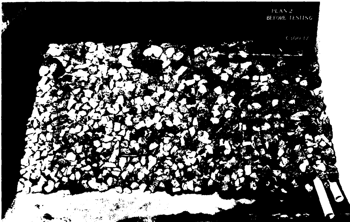
Photo 9. Plan 2, before testing, harbor-side view
