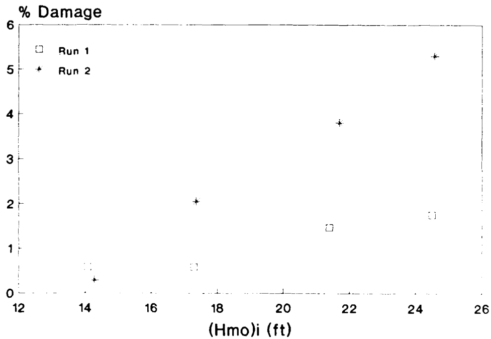
Figure 25. Harbor-side damage, Plan 5, "A-1" Stone
