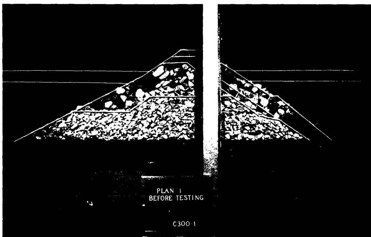
Photo 1. Plan 1, before testing, side view
