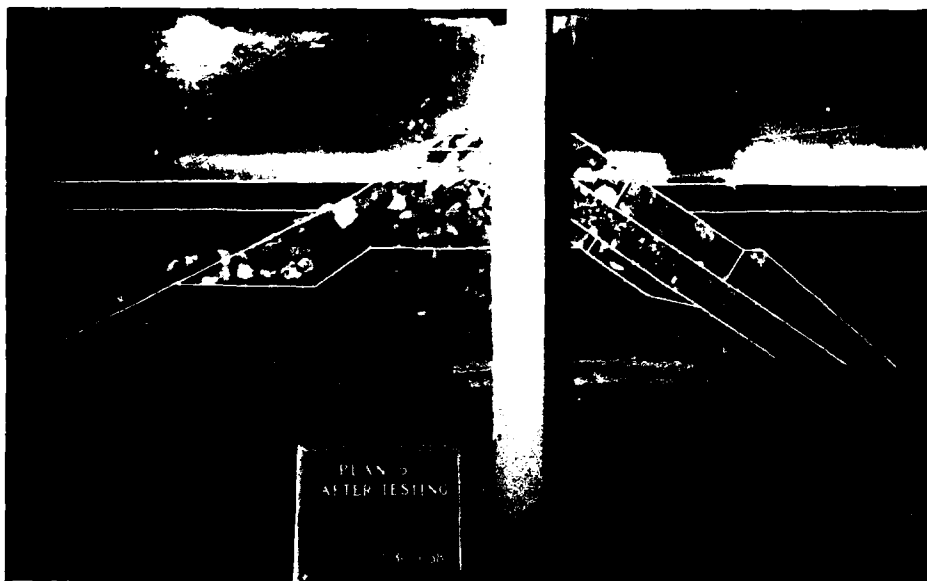
Photo 31. Plan 5, after 24-ft waves, side view
