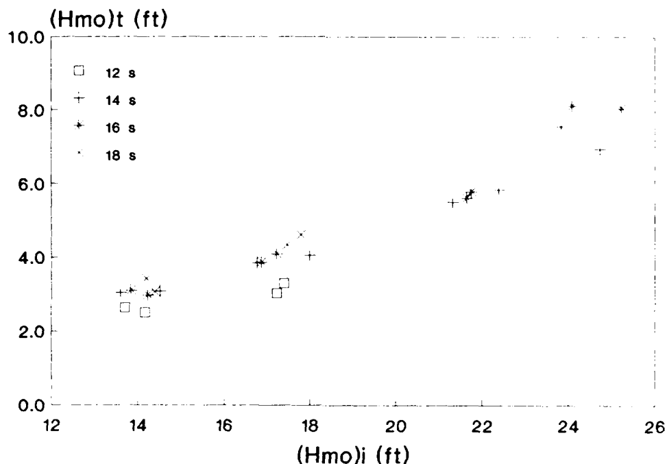
Figure 18. Wave transmission, Plan 3
