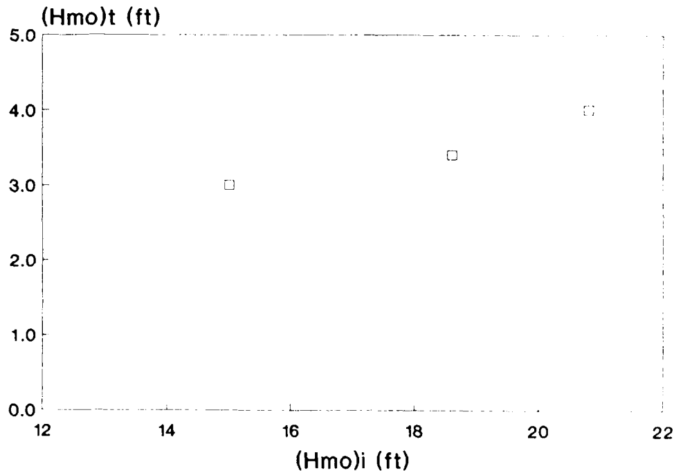
Figure 20. Wave transmission through breakwater, Plan 3
