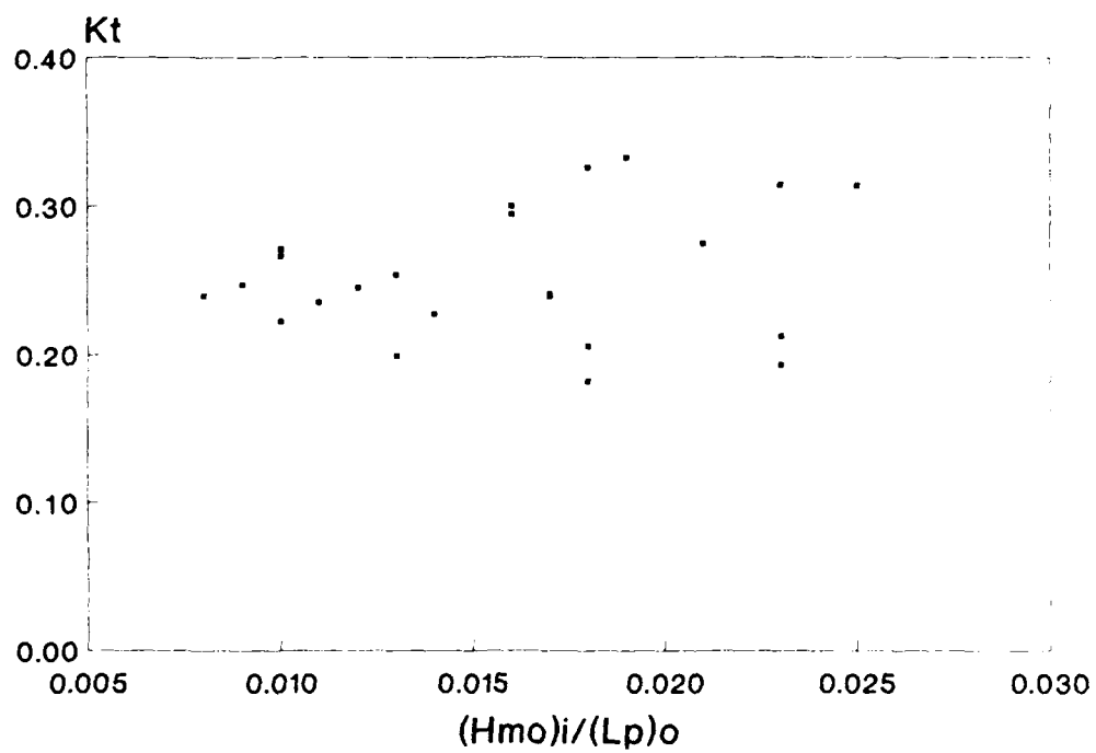
Figure A2. Nondimensional wave transmission, Plan 2
