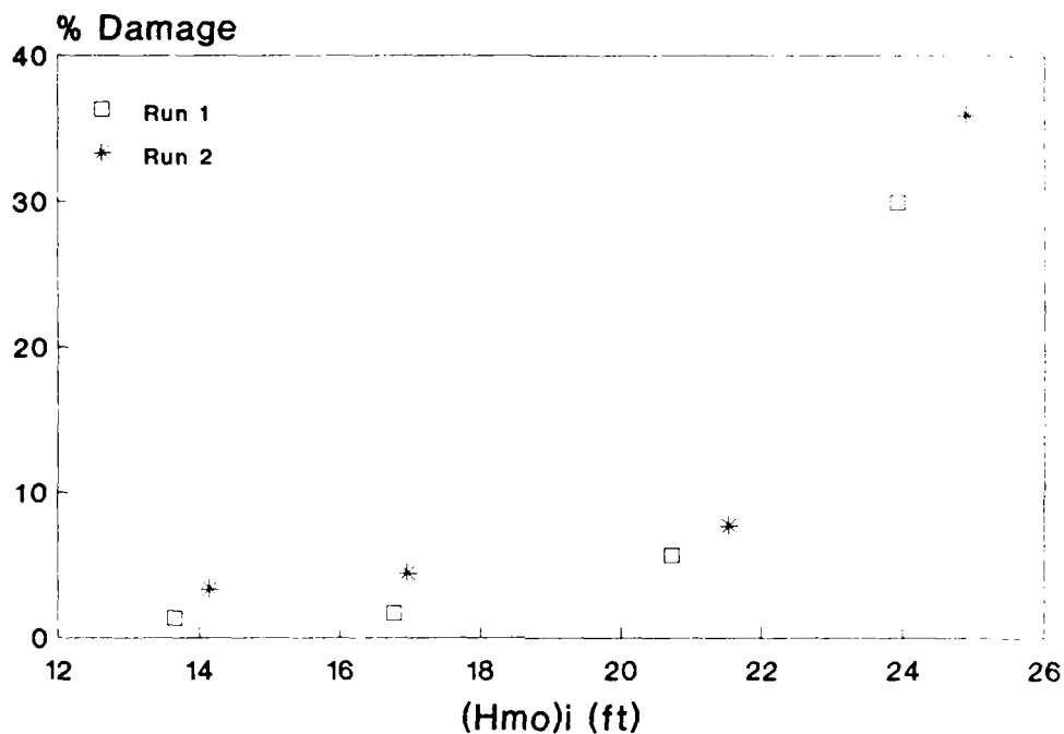
Figure 10. Harbor-side damage, Plan 2, "A" Stone
