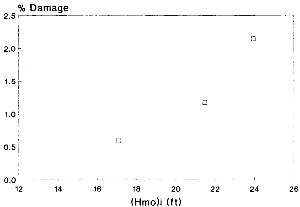
Figure 17. Zone 2 damage, Plan 3
