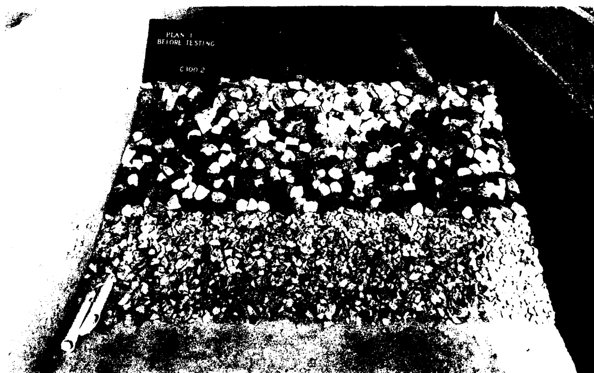
Photo 2. Plan 1, before testing, sea-side view
