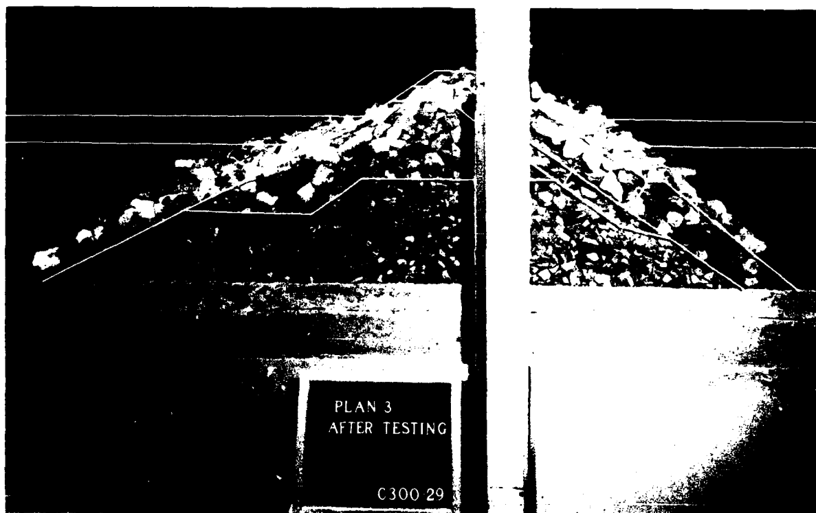
Photo 16. Plan 3, after testing, side view
