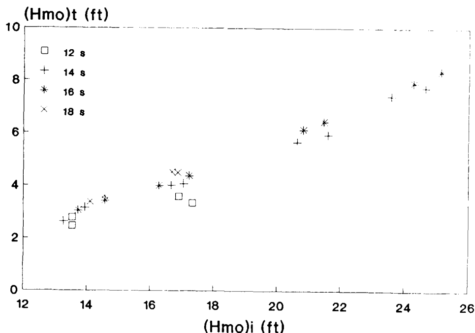
Figure 12. Wave transmission, Plan 2
