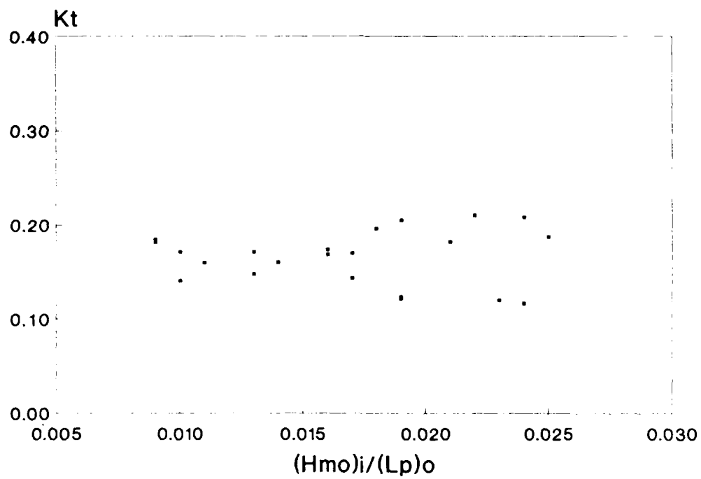
Figure A5. Nondimensional wave transmission, Plan 5
