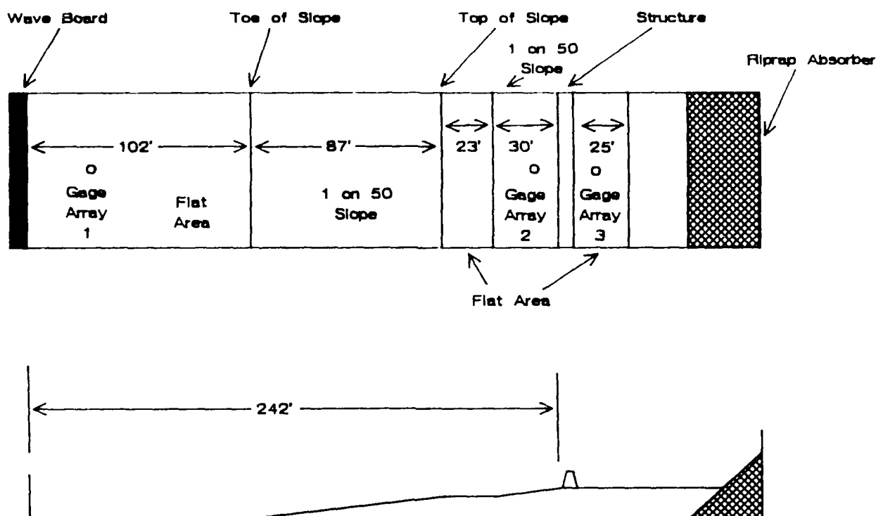
Figure 3. Wave tank used in study
