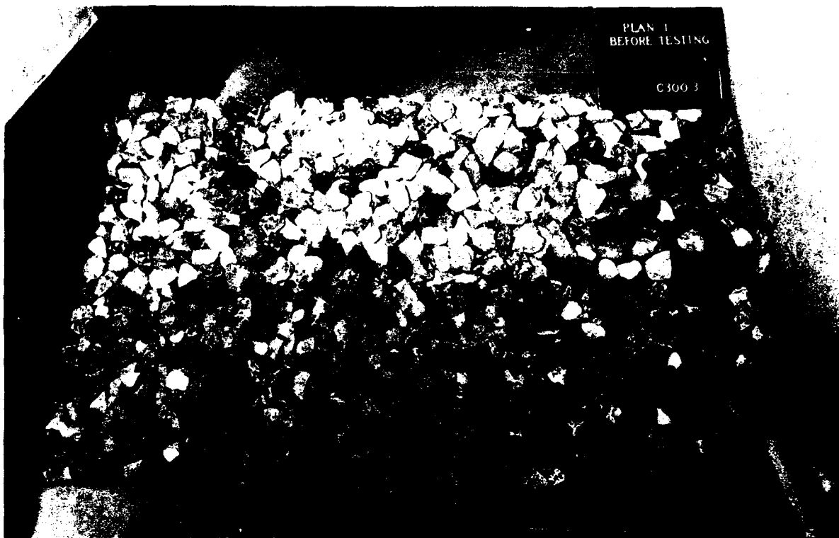
Photo 3. Plan 1, before testing, harbor-side view
