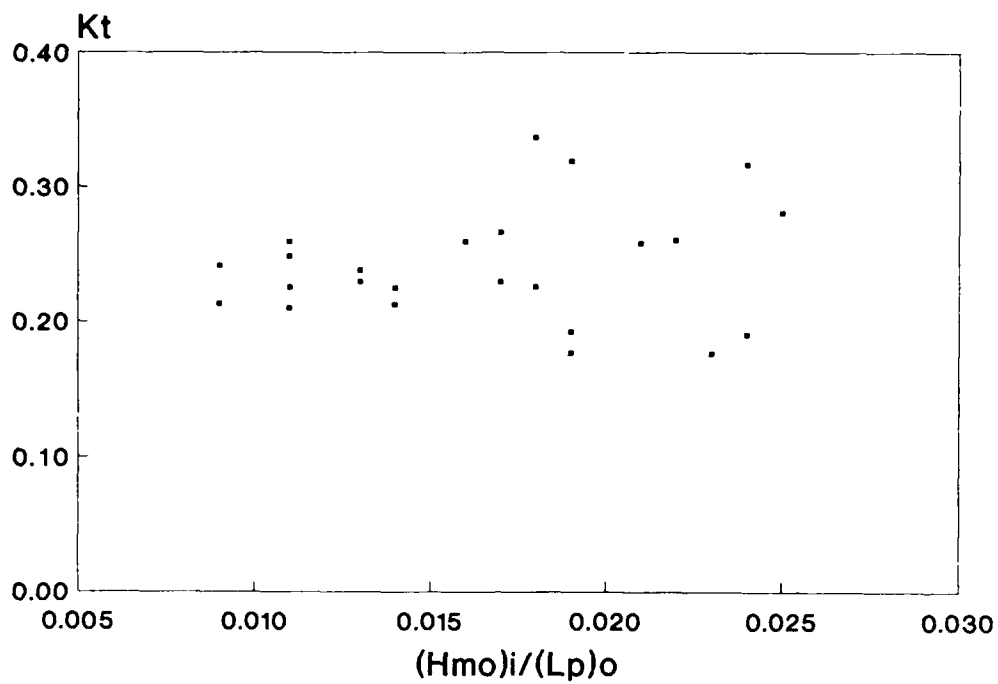
Figure A3. Nondimensional wave transmission, Plan 3
