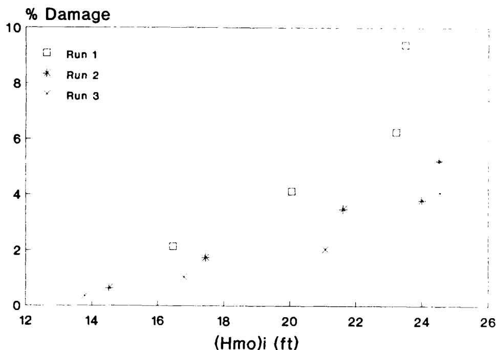
Figure 6. Harbor-side damage, Plan 1
