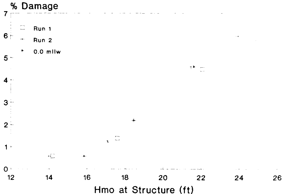
Figure 15. Harbor-side damage, Plan 3
