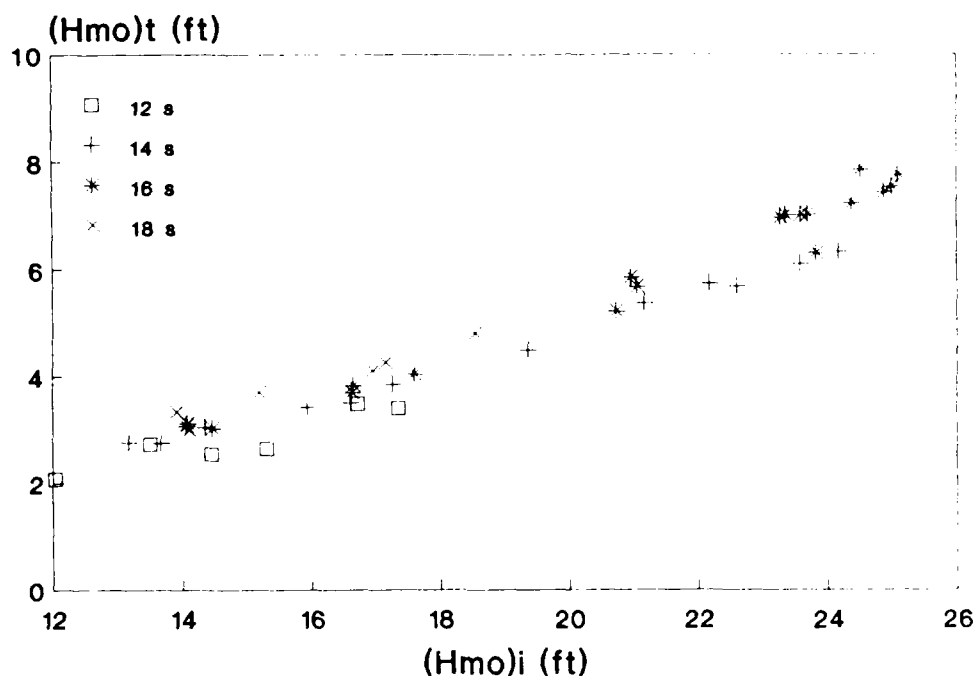
Figure 7. Wave transmission, Plan 1
