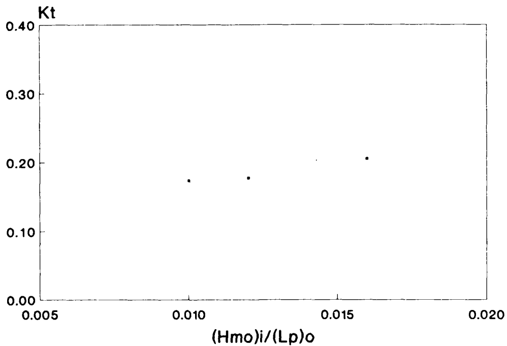
Figure A4. Nondimensional wave transmission, Plan 4
