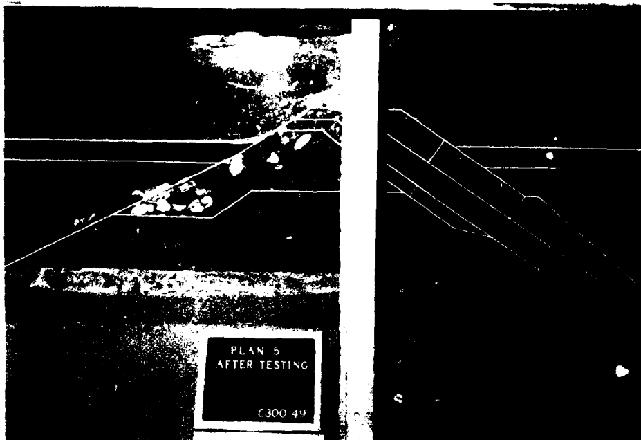
Photo 22. Plan 5, after 13-ft waves, side view
