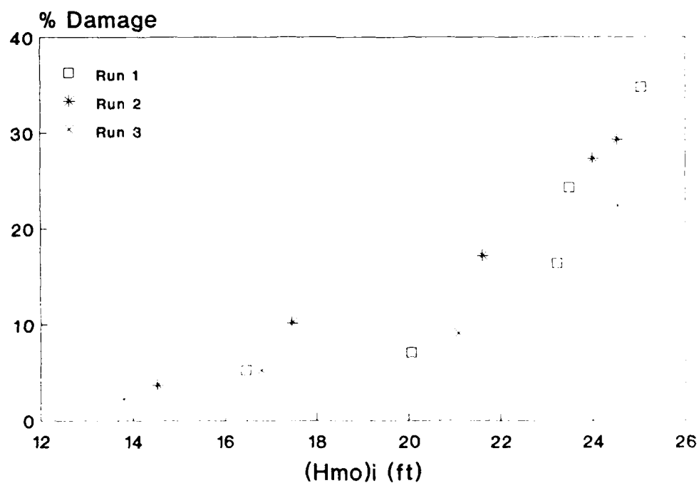
Figure 5. Sea-side damage, Plan 1
