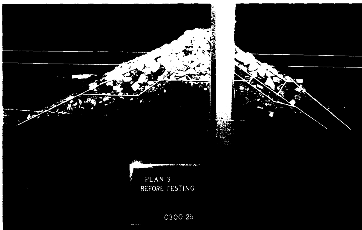
Photo 13. Plan 3, before testing, side view
