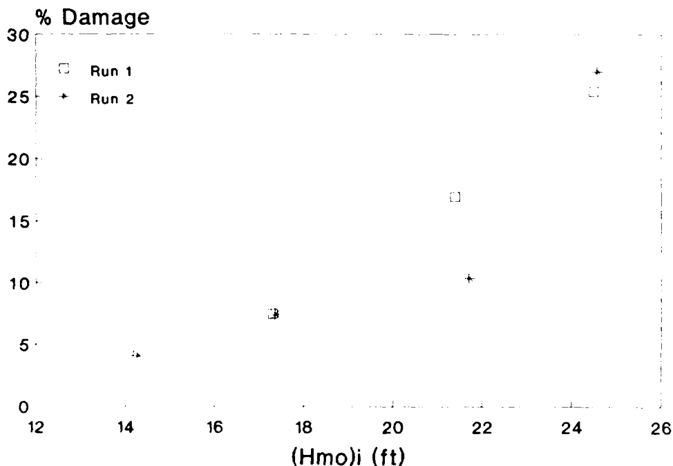
Figure 23. Sea-side damage, Plan 5
