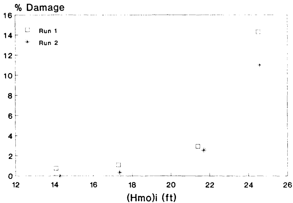
Figure 24. Harbor-side damage, Plan 5, "A" Stone
