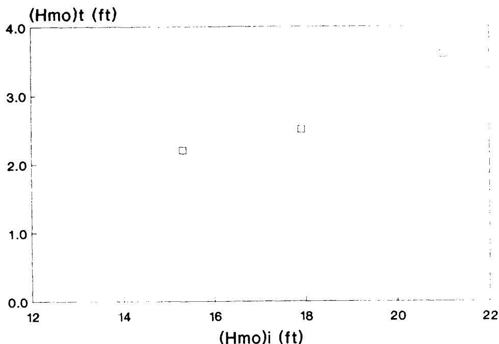
Figure 19. Wave transmission, Plan 3, +0.9 ft mllw
