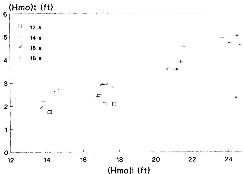
Figure 26. Wave transmission, Plan 5
