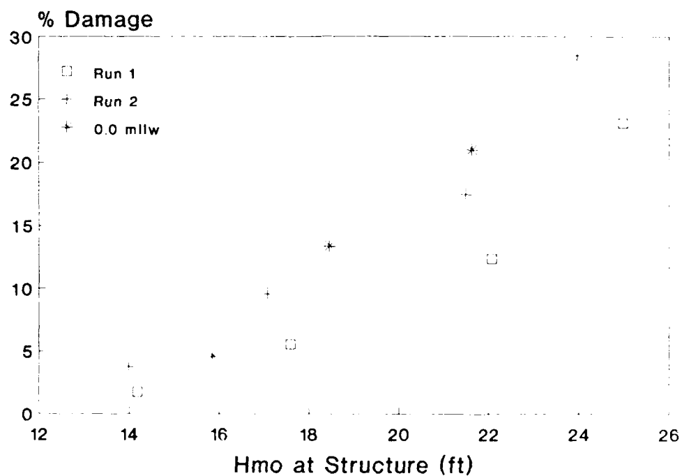
Figure 14. Sea-side damage, Plan 3
