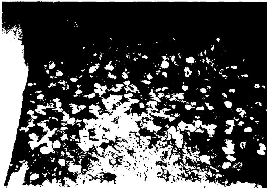
Photo 26. Plan 5, after 16-ft waves, sea-side view
