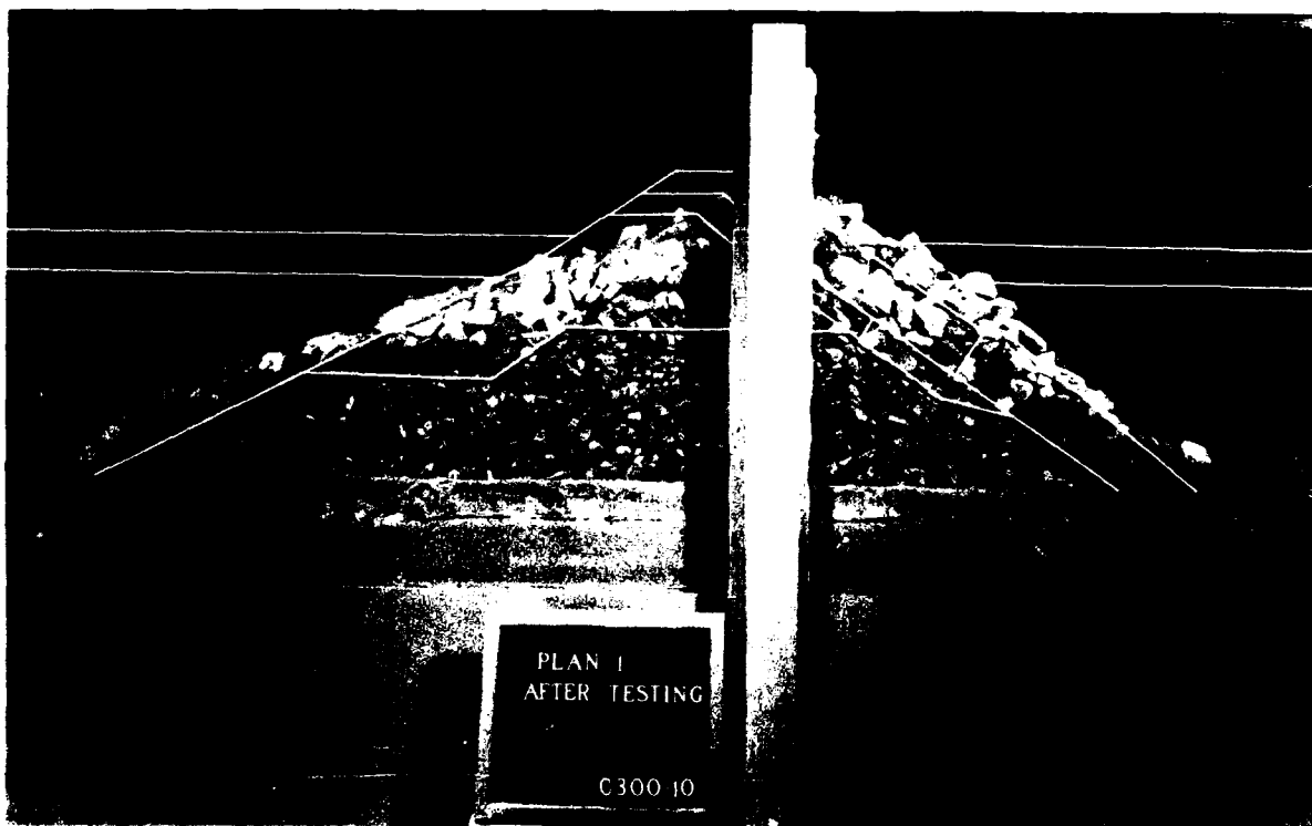
Photo 4. Plan 1, after testing, side view
