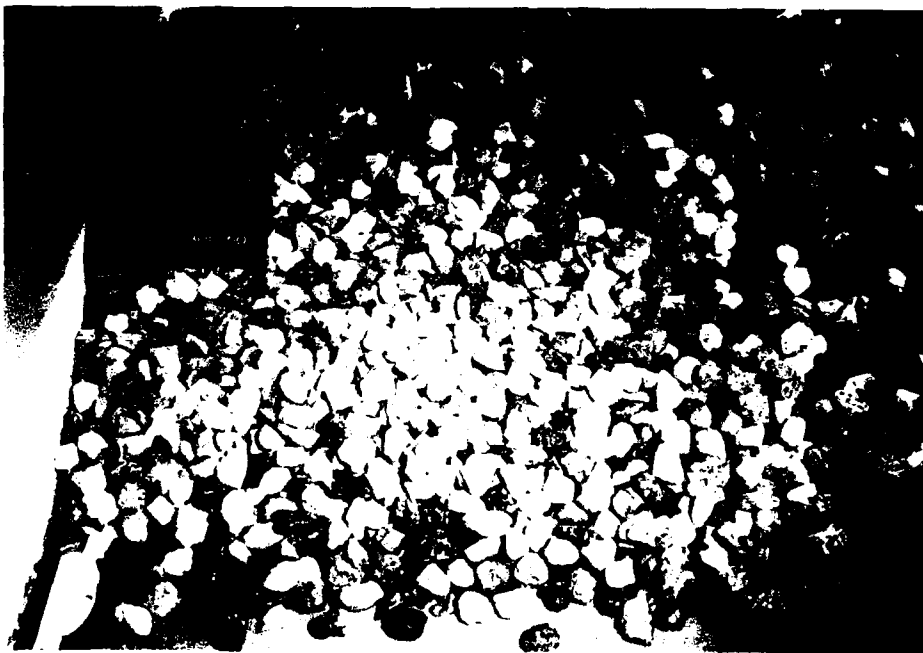
Photo 32. Plan 5, after 24-ft waves, sea-side view
