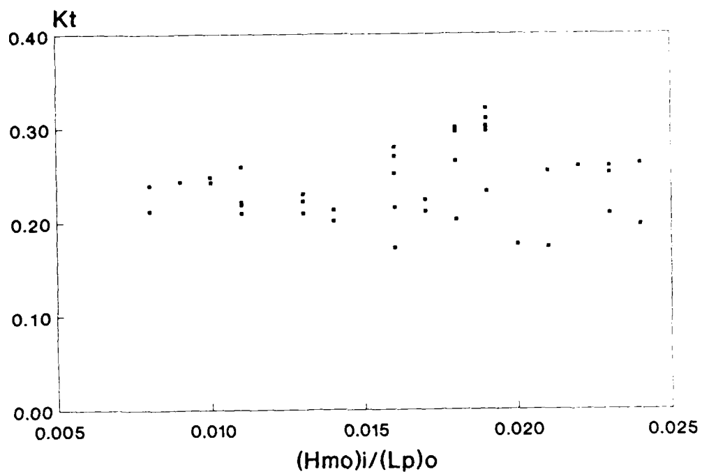
Figure A1. Nondimensional wave transmission, Plan 2
