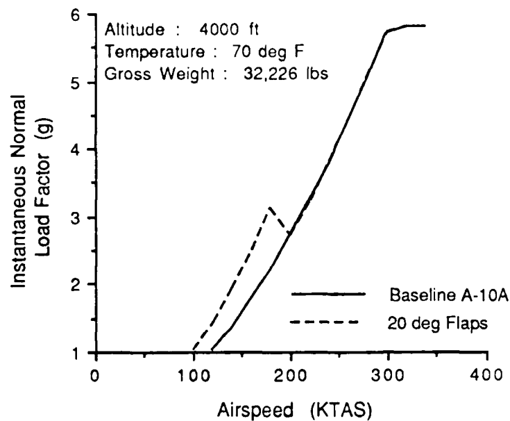
Figure 19. Flap Effect on Normal Acceleration
