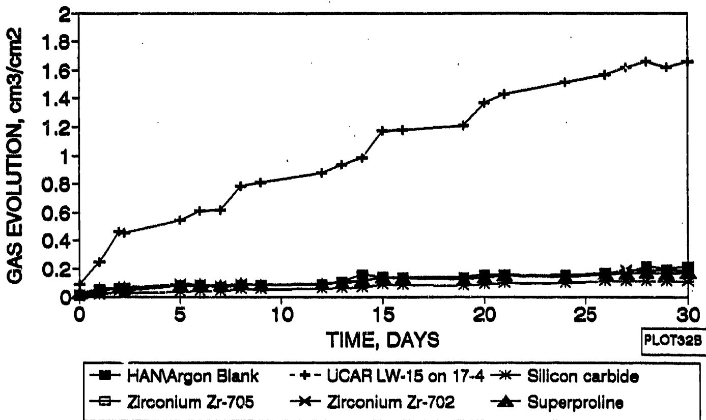
Figure 3.7: Compatibility of Materials in 60.8% HAN at 338 K (65°C)
