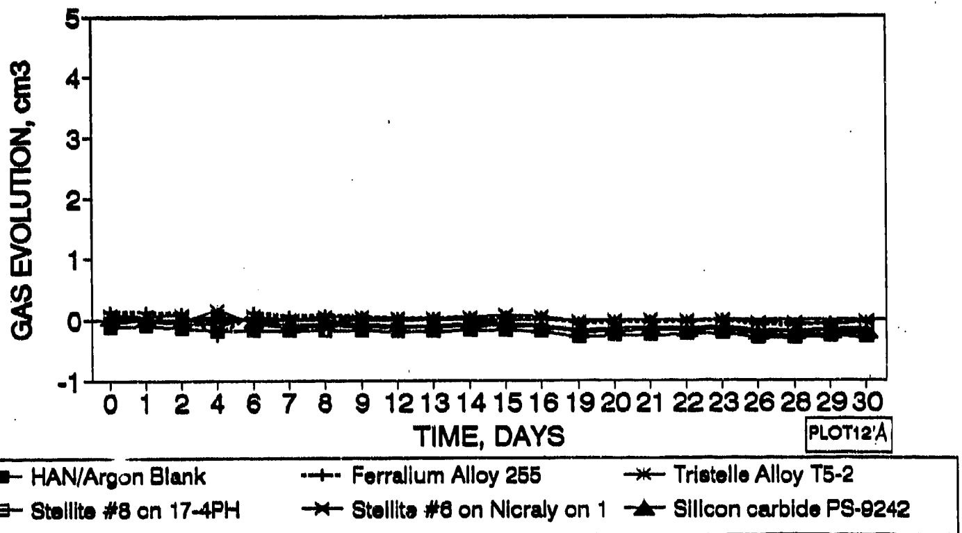
Figure 3.1: Compatibility of Materials in 60.8% HAN at 298 K (25°C)
