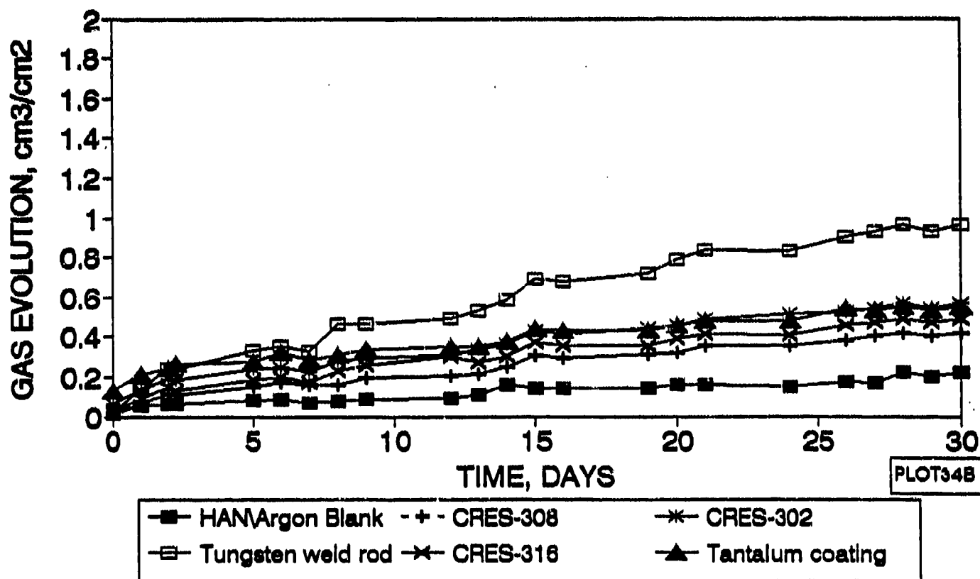
Figure 3.9: Compatibility of Materials in 60.8% HAN at 338 K (65°C)
