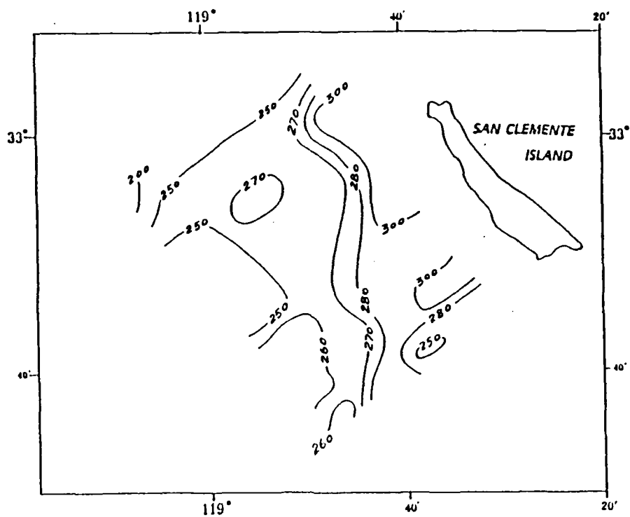
Figure 13a. The depth of 8°C isotherm in the study area
