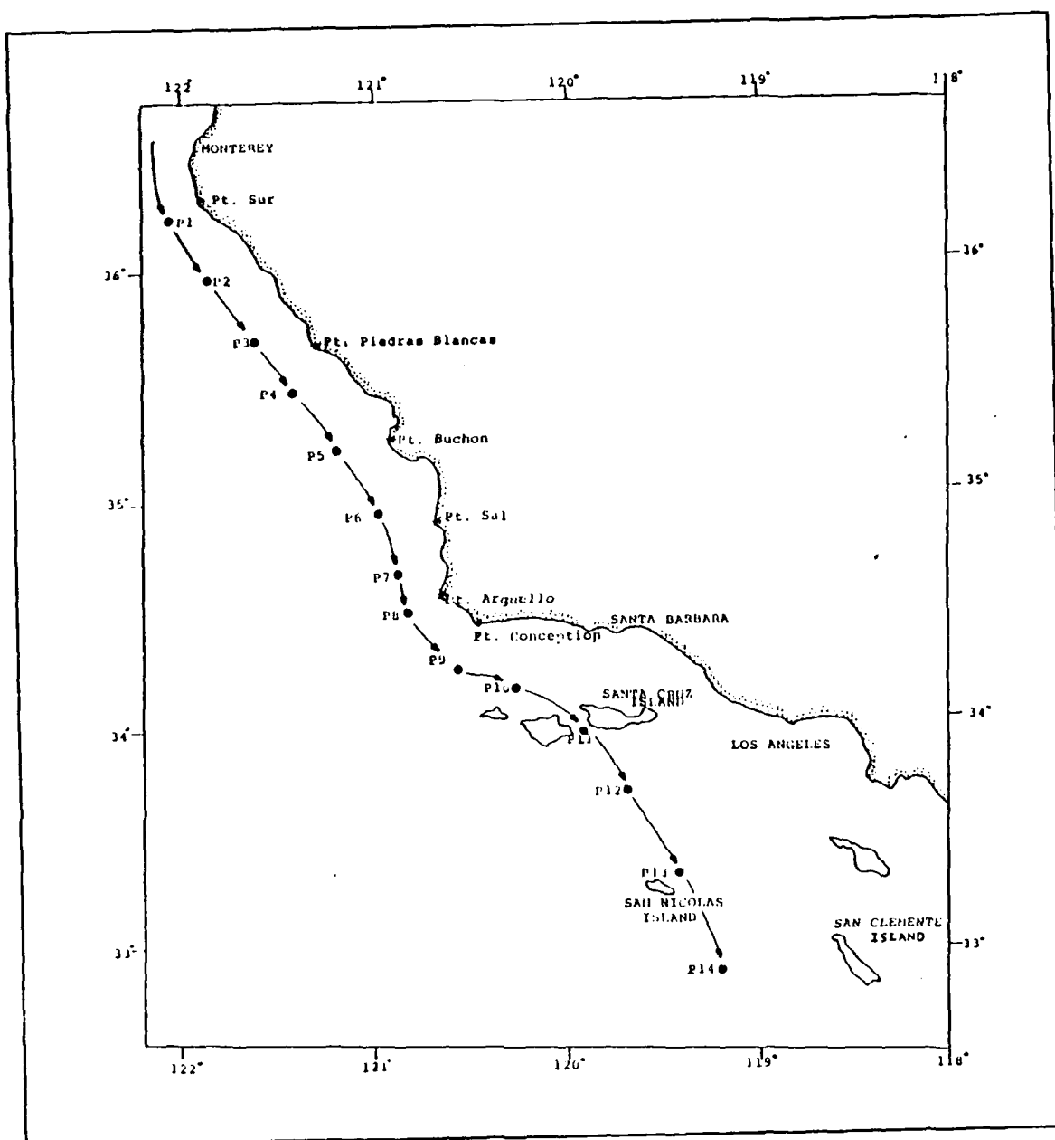
Figure B1. Cruise track followed during the steam from the Moss Landing to San Clemente Island during the cruise SCBE-II, 2-6 September, 1989. The solid circle denotes the location of XBT sounding.
