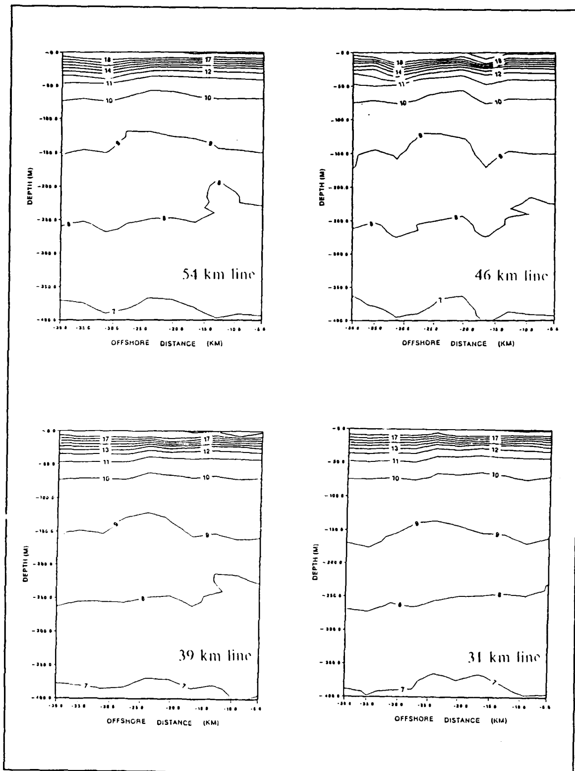
Figure 14a. Vertical cross-section of temperature at the 54 km, 46 km, 39 km and 31 km line in figure 9
