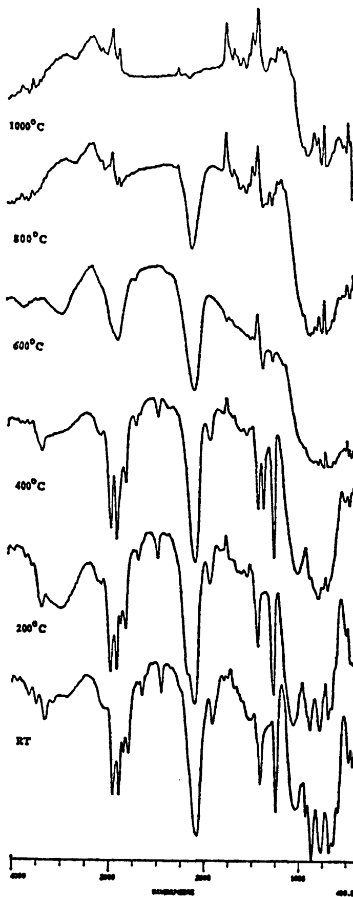
Figure 6. DRIFT Spectra of -\text{[HSiMe]}_x- Heated to Selected Temperatures
