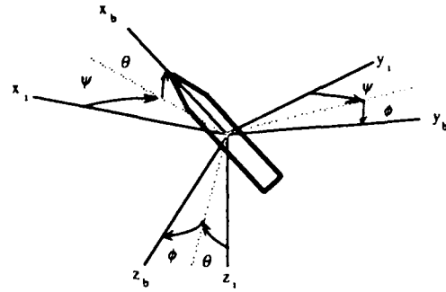
Figure 1: Axes systems.
