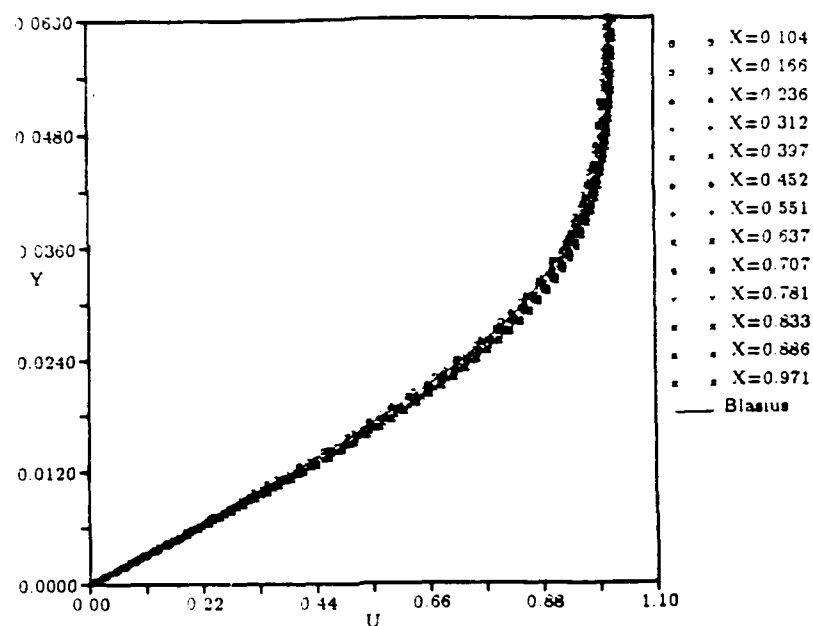
Fig. 10: Velocity profiles for a Blasius boundary layer.
