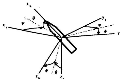
Figure 1: Axis systems.
