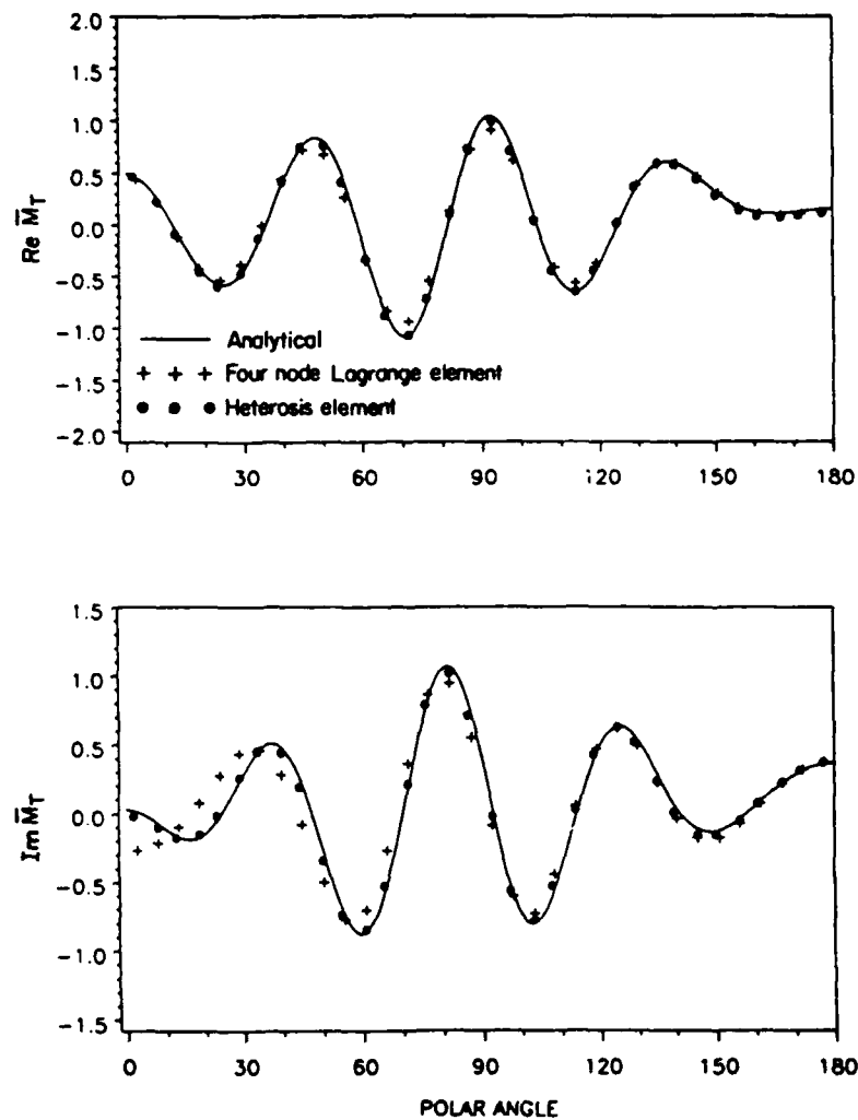
Fig. 4. Variation of tangential moment (parameters are the same as in Fig. 3).
