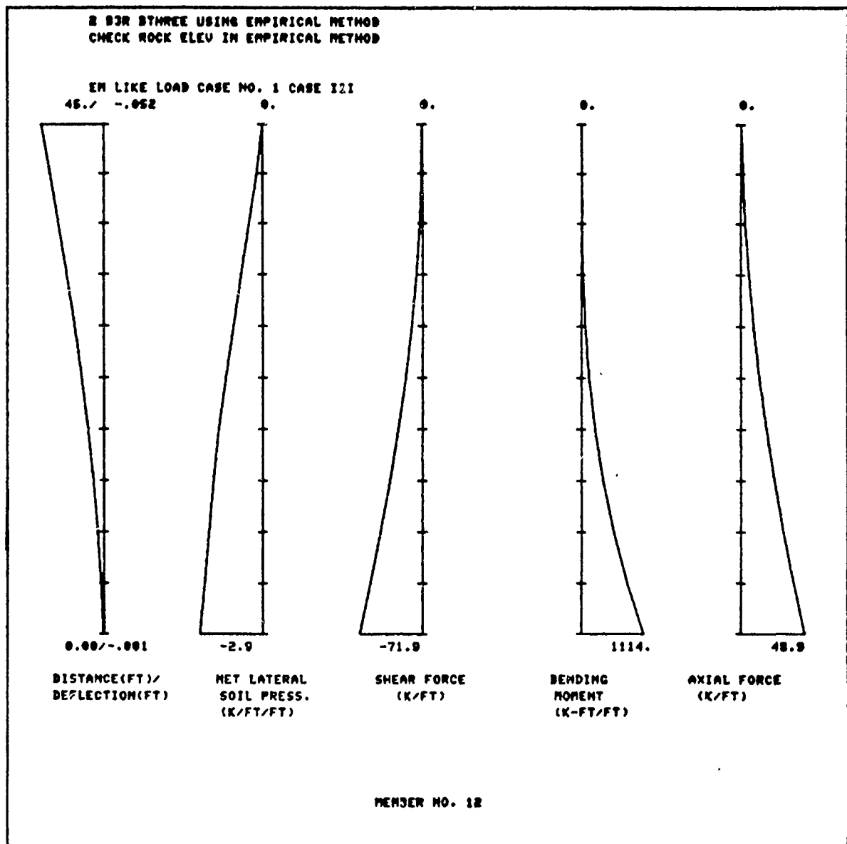
Figure 23. Sample member force plot for wall member
