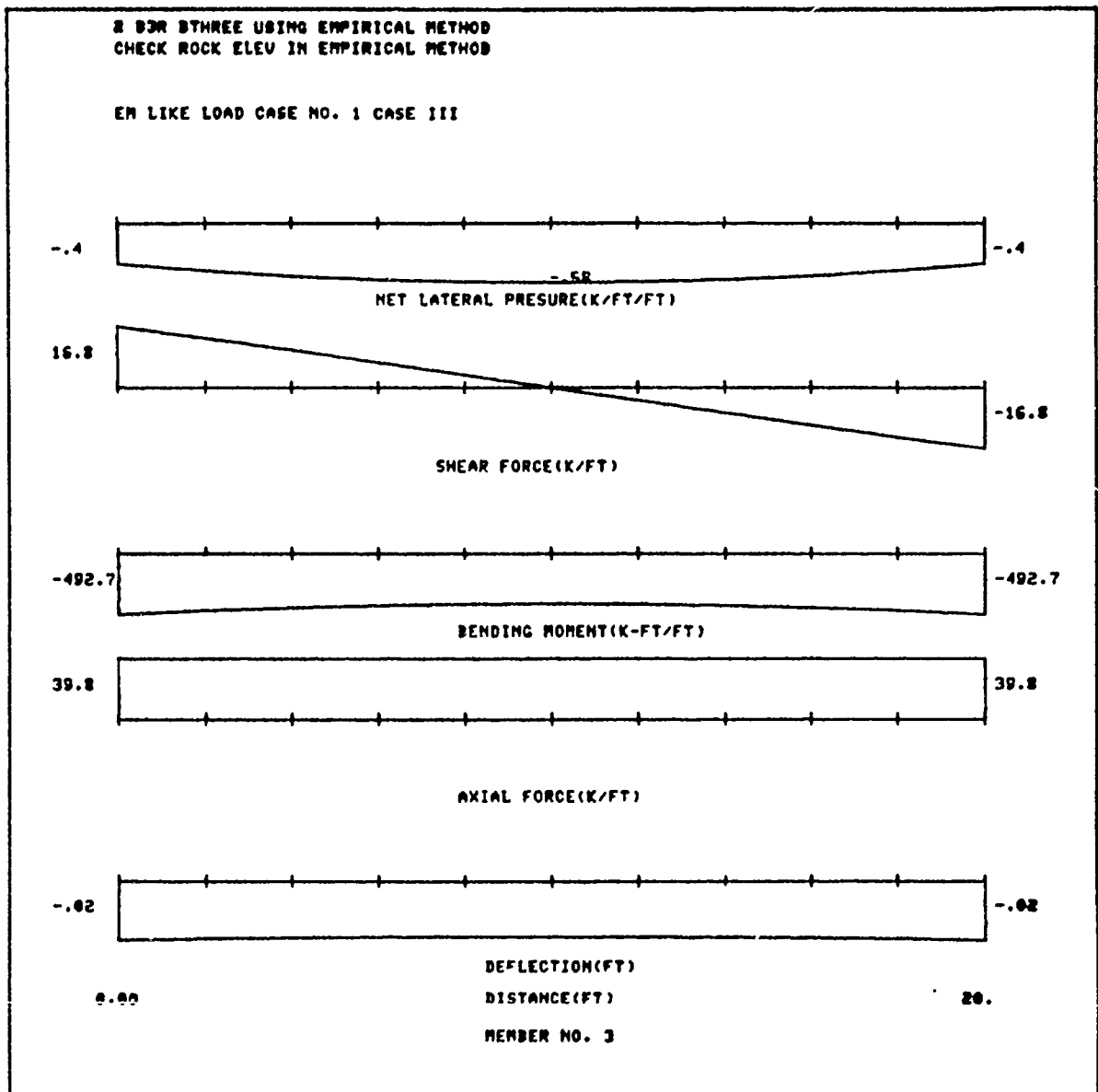
Figure 22. Sample member force plot for slab member
