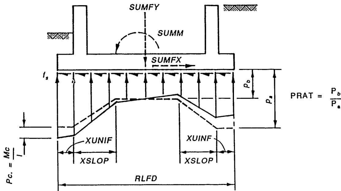
Figure 12. Empirical foundation pressures
