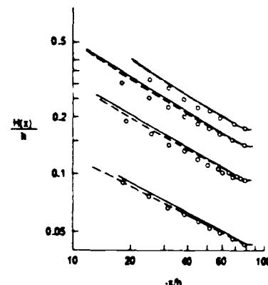
Fig. 6. Normalized amplitude of solitary waves in converging channel with h = 30 cm and initial amplitudes H_0/h = 0.043, 0.093, 0.140, \text{ and } 0.174 . Circles show data from CMM, solid curves show the total wave train, and dashed curves show the incident wave alone.
