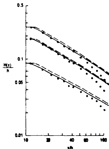
Fig. 5. Normalized amplitude of solitary waves in diverging channel with h = 20 cm and initial amplitudes H_0/h = 0.088, 0.185, \text{ and } 0.259 . Circles show data from CMM, solid lines show the total wave train, and dashed lines show the incident wave alone.
