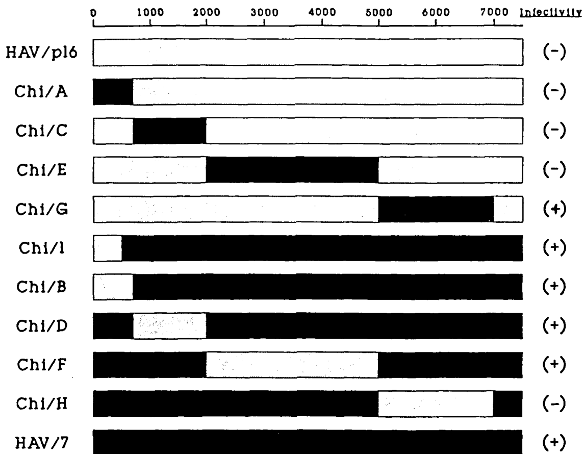
Figure 4. Chimeric genomic-length cDNA constructs containing regions derived from cell culture-adapted but virulent p16 HM175 (stippled regions), and cell culture-adapted, attenuated p35 HMI75 virus (pHAV/7 cDNA, shaded regions). Whether or not infectious virus was produced following transfection of BS-C-1 cells with related RNA transcripts is indicated to the right.
