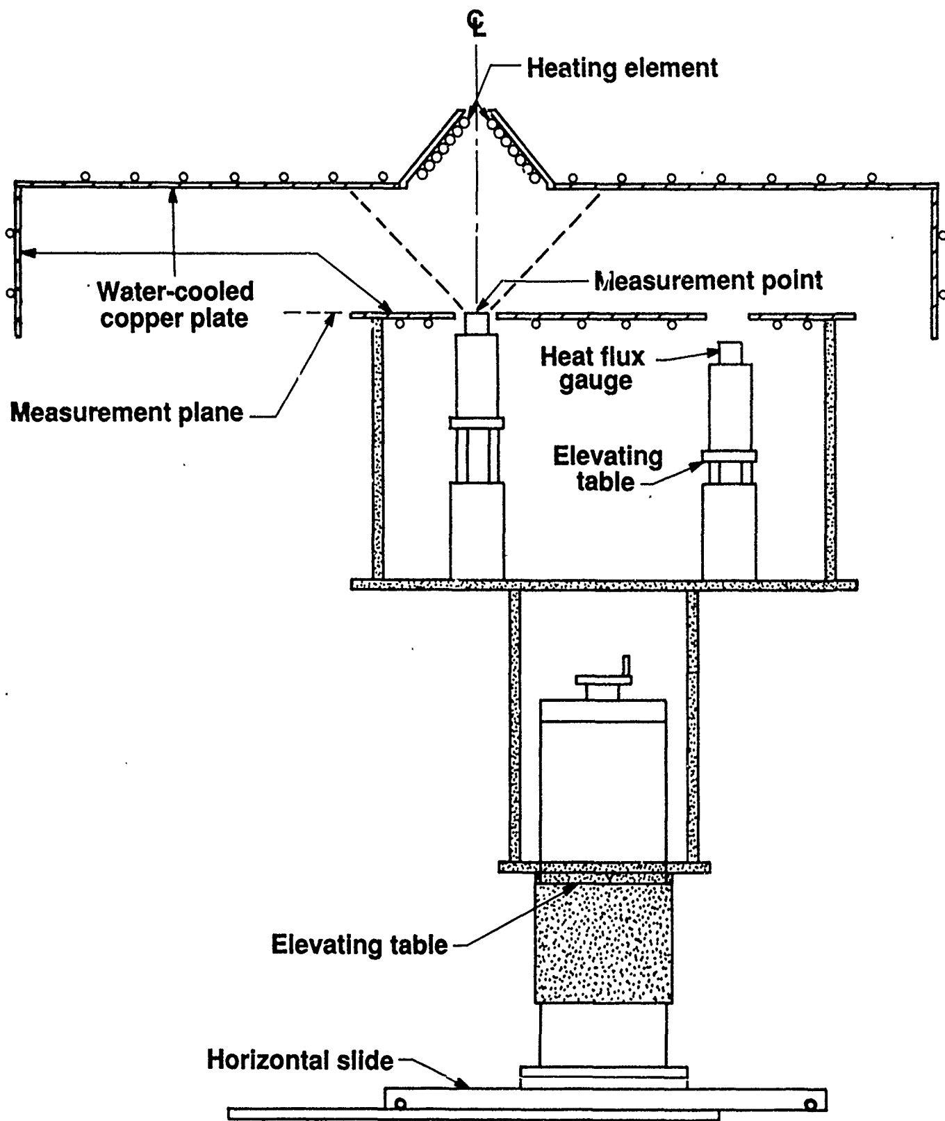
FIGURE 6. CFR CALIBRATION APPARATUS FOR HEAT FLUX SENSORS
