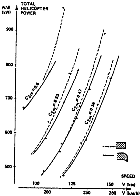
Fig. 44. AS-365N performance improvement in forward flight with parabolic sweptback tips, from [35]
