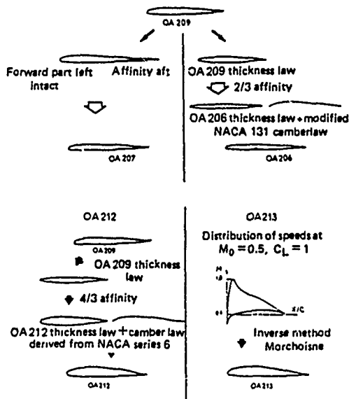
Fig. 55. Design methodology of OA-207, OA-206, OA-212 and OA-213 airfoils, from [78]
