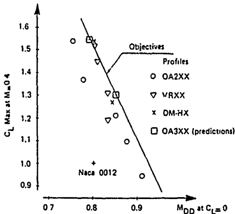
Fig. 56. Main aerodynamic characteristics of new airfoils for helicopter blades
