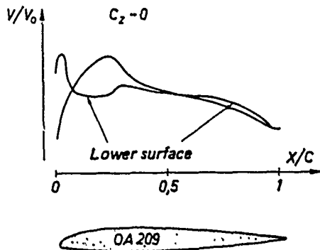
Fig. 54. Design of OA-209 airfoil, from [78]
