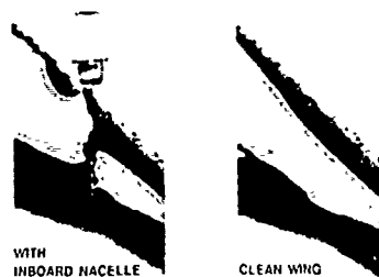
CFD ANALYSIS OF AN ENGINE INSTALLATION M = 0.86 Surface Mach Number Contours
