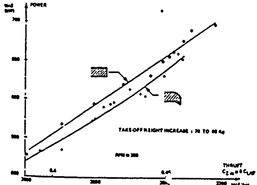
Fig. 45. AS-365N performance improvement in hover with parabolic sweptback tips, from [35]
