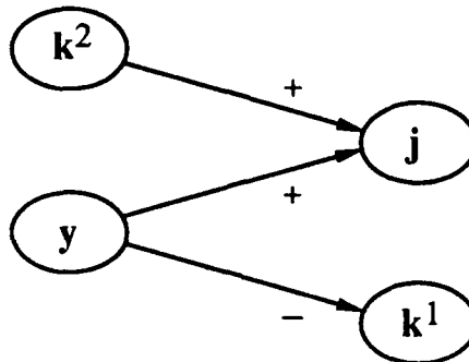
FIGURE 4. The choice of links to reverse before reducing y determines the strength of the final result.
