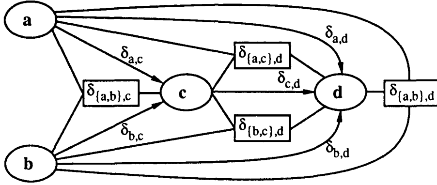
FIGURE 3. A fragment of QPN G before performing a QPN transformation. The relations on d holding in G' after reducing c from the network are given by the update equations (2) and (3). Reversing the link from c to d results in G'' , described by equations (4–6).
