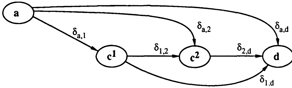
FIGURE 6. General QPN fragment for analyzing the order-invariance of reducing c^1 and c^2 .
