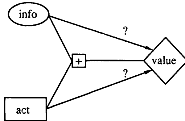
FIGURE 2. The generic decision model reduced to three variables.
