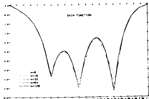
Figure 2 Gain Function h_{\alpha, \alpha}^1(\cdot) ( \alpha = 0.3 , C(x) = (z(0.3), z(0.5), z(0.75)) )
