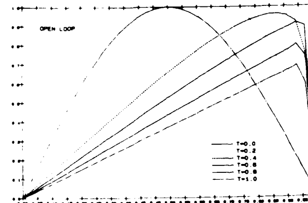
Figure 12 Open Loop ( N=32, Re=100, z_0(x) = \sin \pi x )
