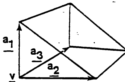
Figure E-7: Right Angle Wedge (WED)
