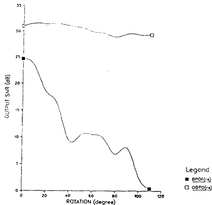
Figure 3-15: Output SNR (vs) rotation for BPOF(re) and OBPOF(re) using centered tank image.
