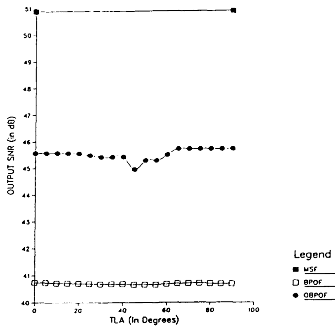
Figure 3-5: Output SNR (vs) TLA for BPOF and Optimal BPOF for non-centered tank.
