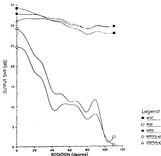
Figure 3-16: Output SNR (vs) rotation for MSF, POF, OPOF, BPOF(re), and OBPOF(re) using centered tank image.
