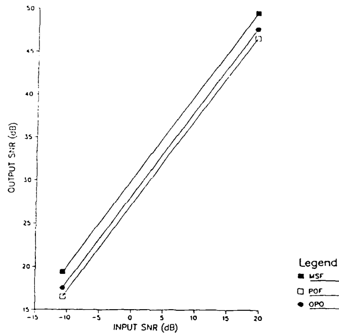
Figure 2-23: Output SNR (vs) input SNR for tank-APC.
