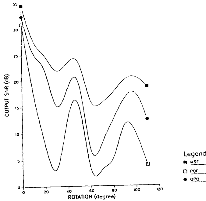
Figure 2-18: SNR (vs) input rotation for pliers image for MSF, POF, and OPOF.
