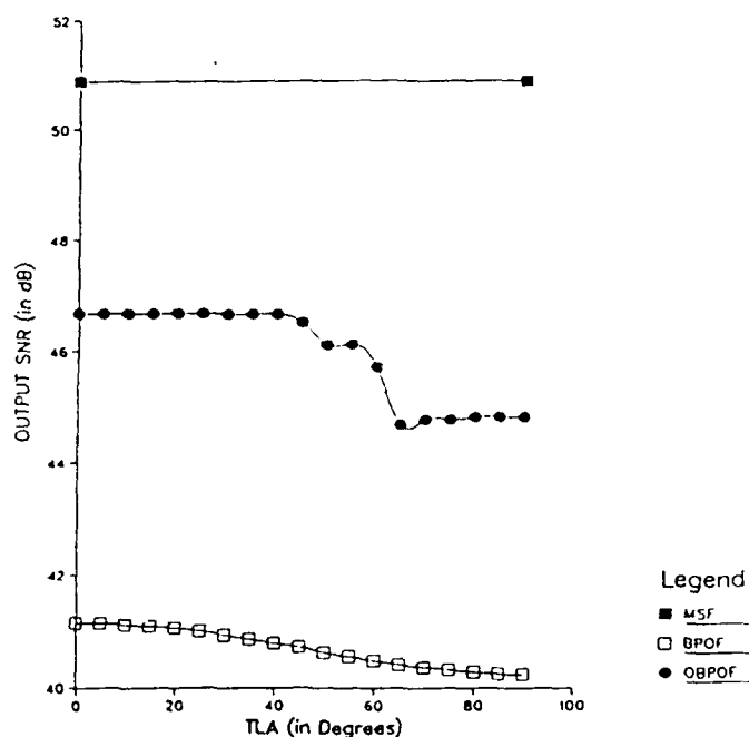
Figure 3-2: Output SNR (vs) TLA for BPOF and Optimal BPOF for centered tank.
