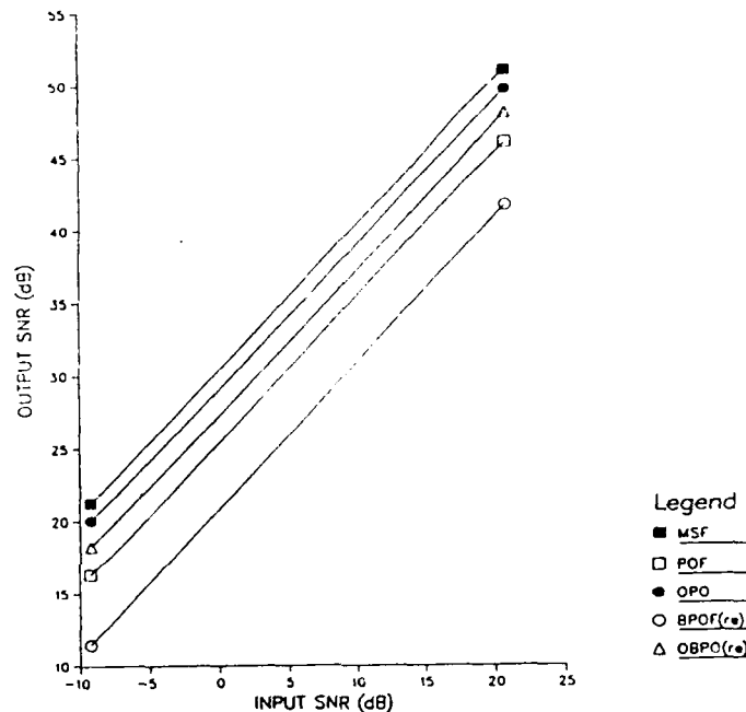
Figure 3-9: Output SNR (vs) input SNR for MSF, POF, OPOF, BPOF(re), and OBPOF(re) using centered tank.
