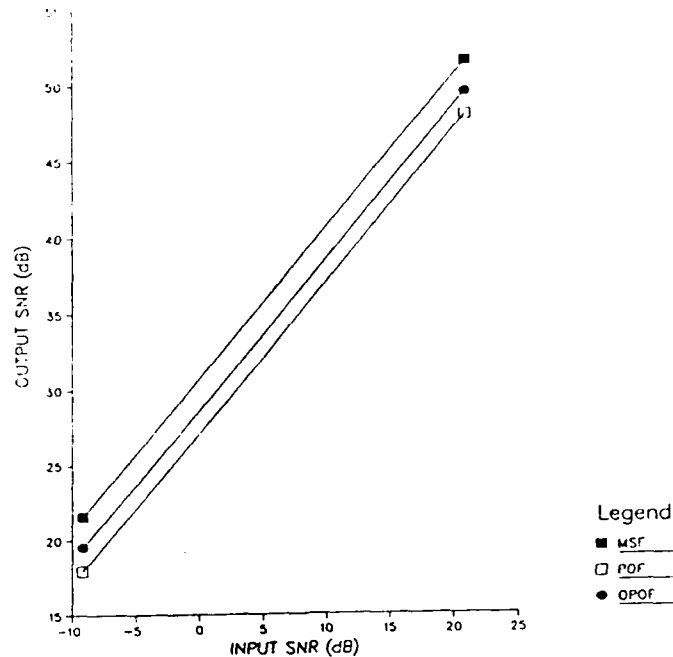
Figure 2-15: Output SNR (vs) input SNR for pliers image.
