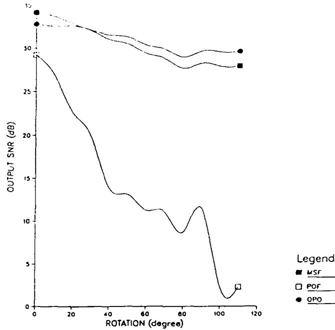
Figure 2-17: SNR (vs) input rotation for tank image for MSF, POF, and OPOF.
