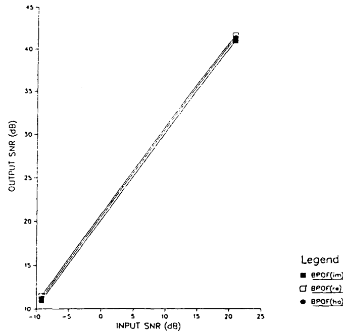
Figure 3-7: Output SNR (vs) input SNR for BPOF(re), BPOF(ha), and BPOF(im) using centered tank.
