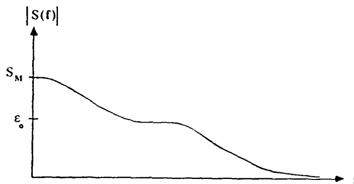
Figure 2-1: Hypothetical signal spectrum.
