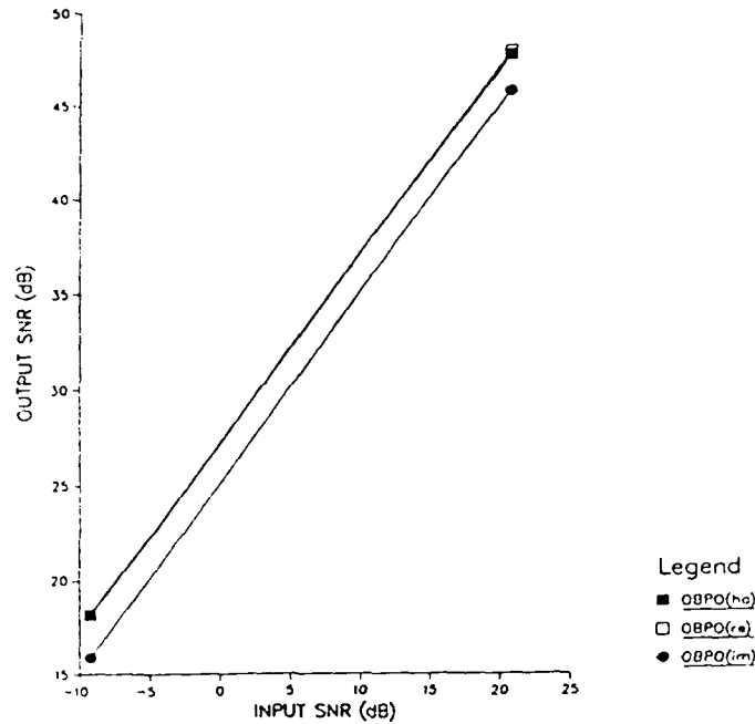
Figure 3-8: Output SNR (vs) input SNR for OBPOF(re), OBPOF(ha), and OBPOF(im) using centered tank.
