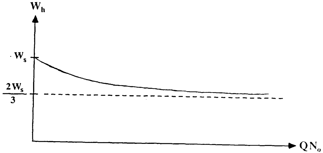
Figure 2-24: Plot of W_h as a function of Q N_0 .
