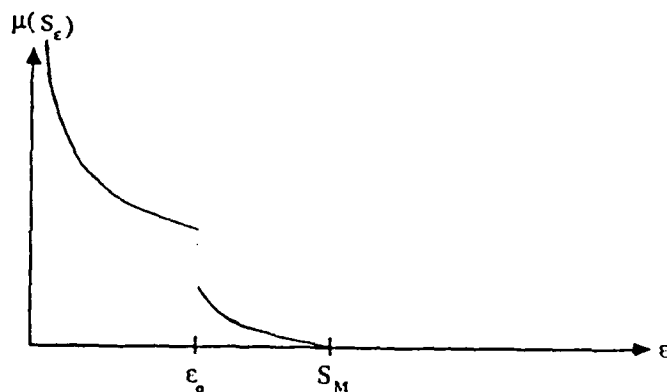
Figure 2-2: Lebesgue measure of S_\epsilon for above spectrum.
