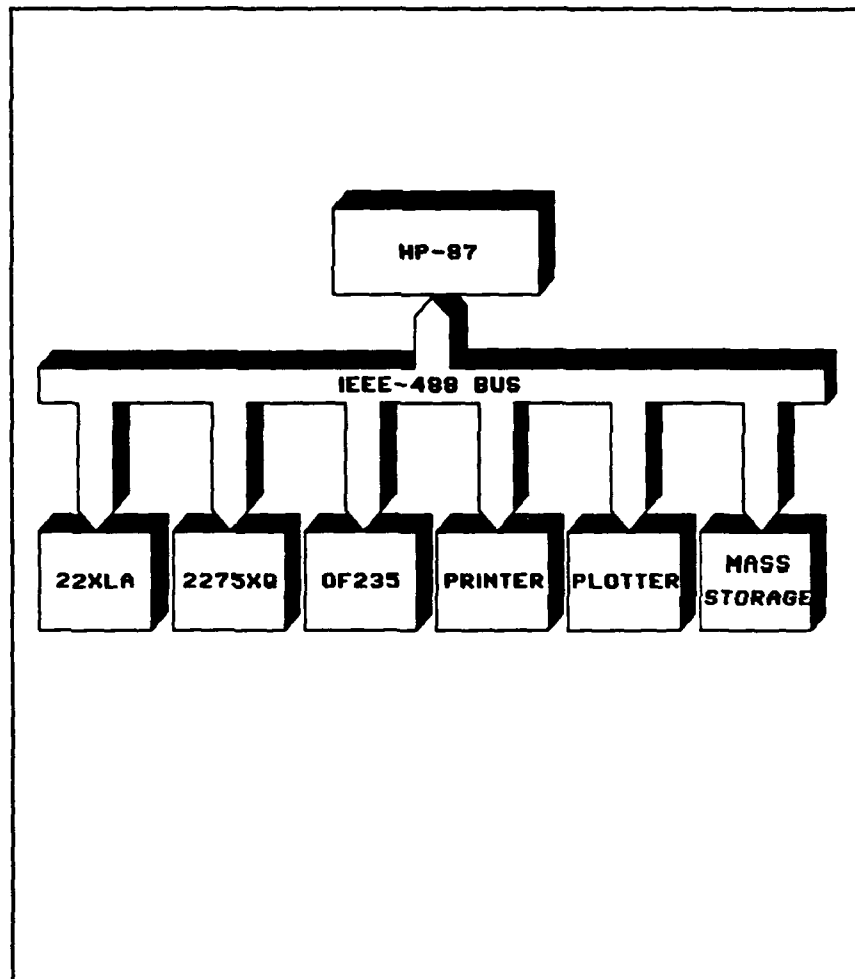
Figure 2. System configuration
