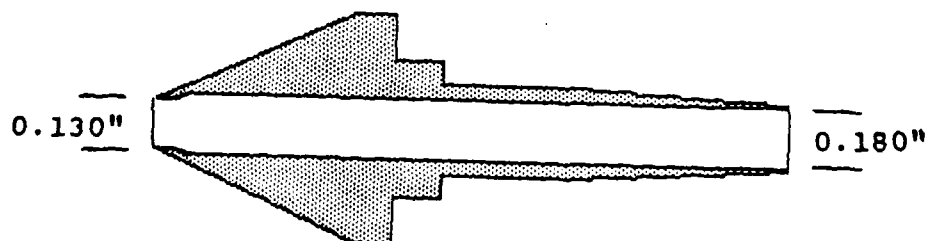
Figure 4.2 Cutaway View of Tip Modification
