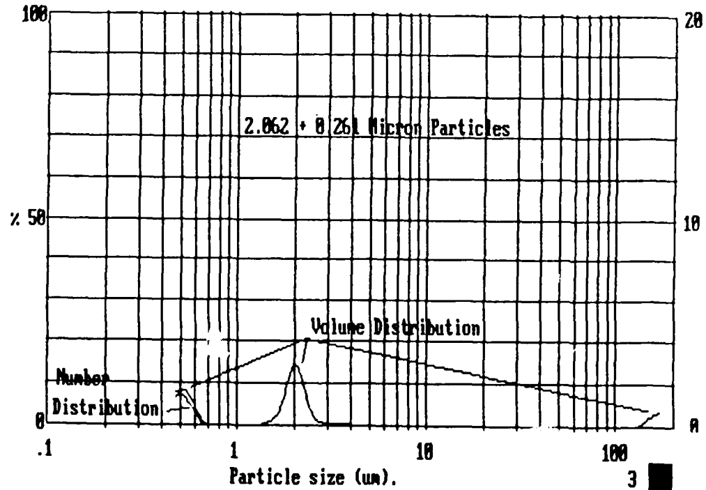
Figure A.5 Bi-Modal Sample (2.062 + 0.261 Microns)
