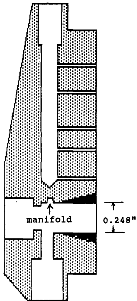
Figure 4.3 Cutaway View of Probe Head Modification
