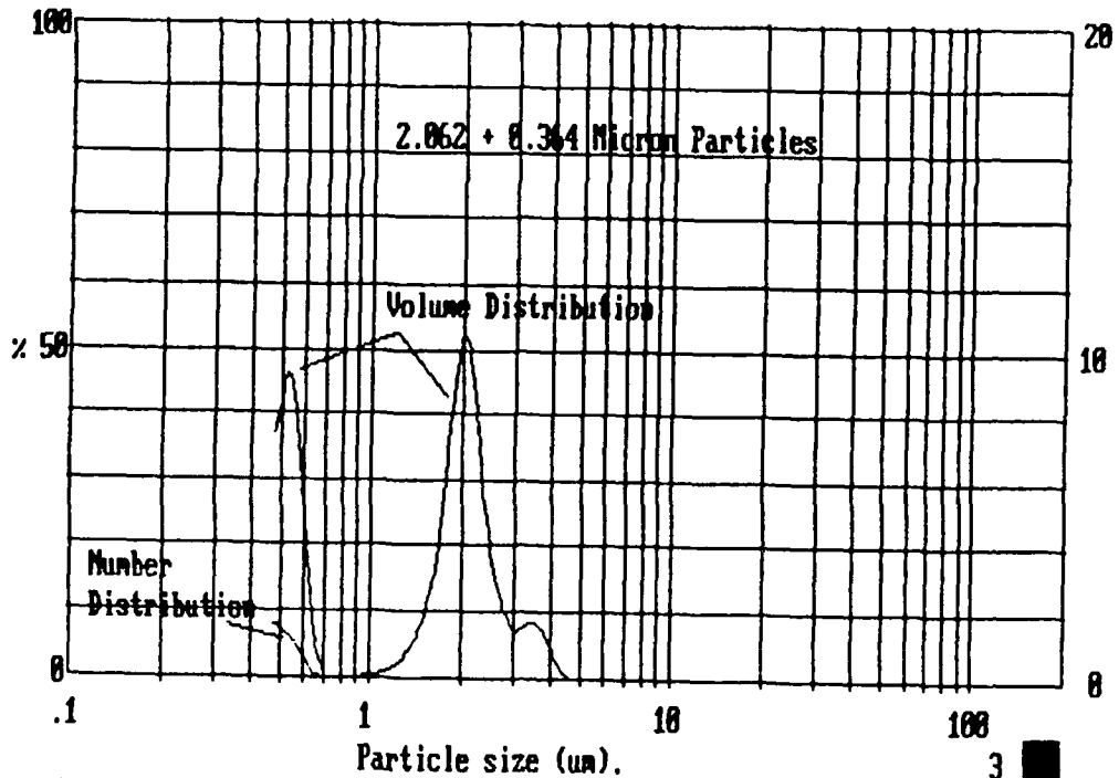
Figure A.4 Bi-Modal Sample (2.062 + 0.364 Microns)
