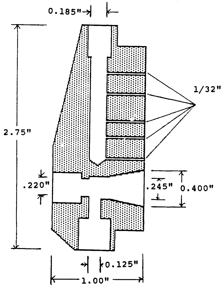
Figure 2.5 Cutaway View of Probe Head
