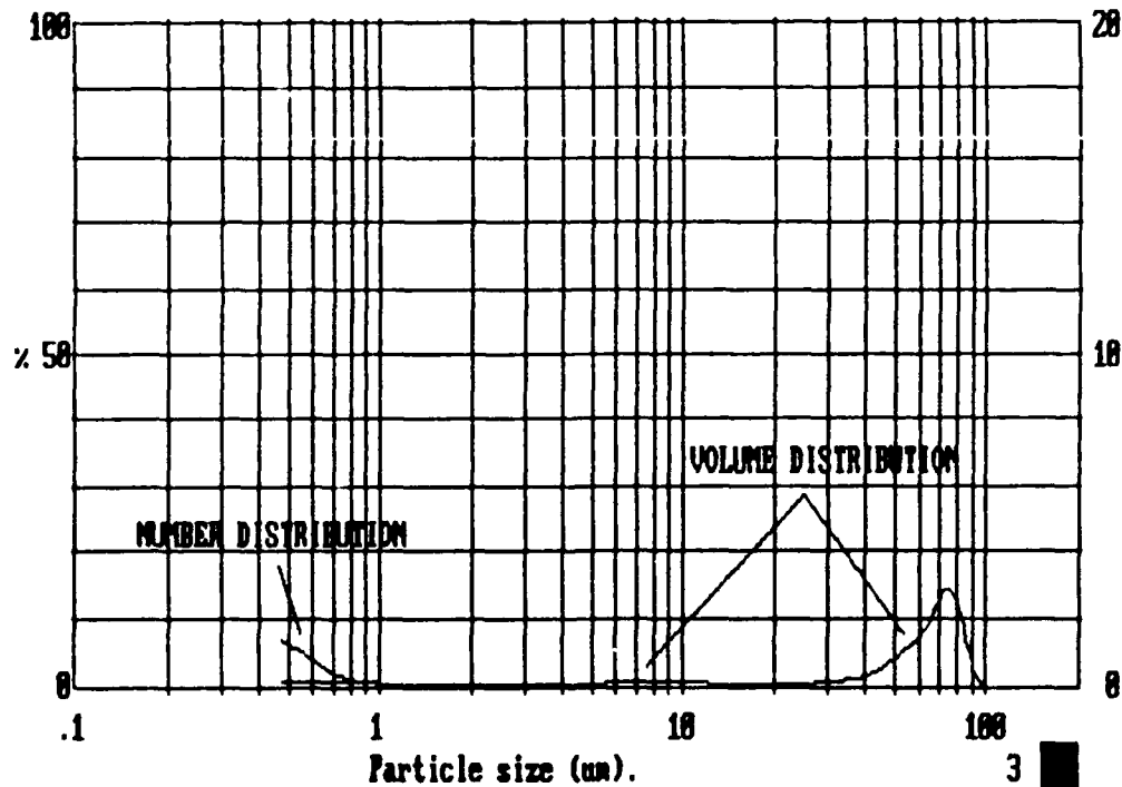
Figure 4.11 Mastersizer Results - Test Firing
