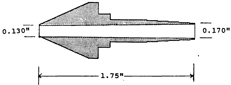
Figure 2.4 Cutaway View of Tip Interior
