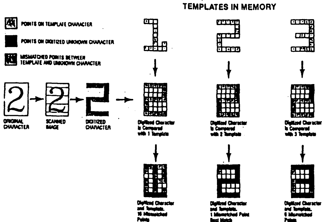
Figure 3-7. Matrix Matching
