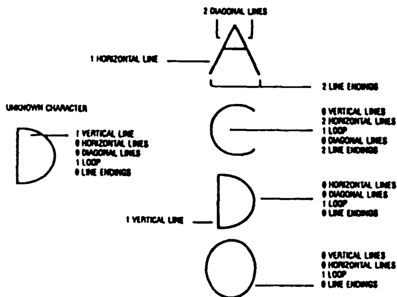
Figure 3-8. Feature Extraction
