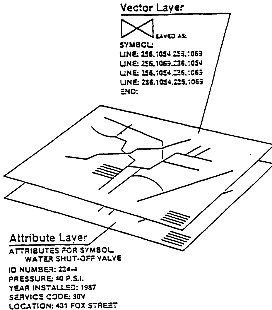
Figure 3-4. Vector Technology
