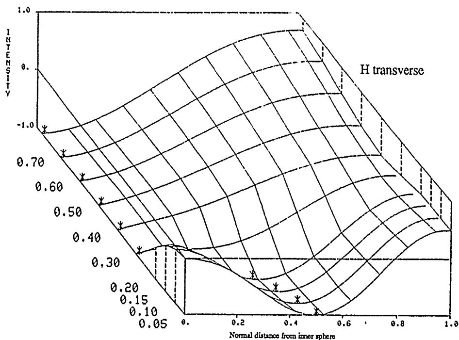
Figure 68. Distribution of the normalized transverse magnetic field component in the concentric spherical cavity as a function of the inner to outer conductor radii, R = bla , for the TM 32 mode. Asterisk indicates peak value of field with d .
