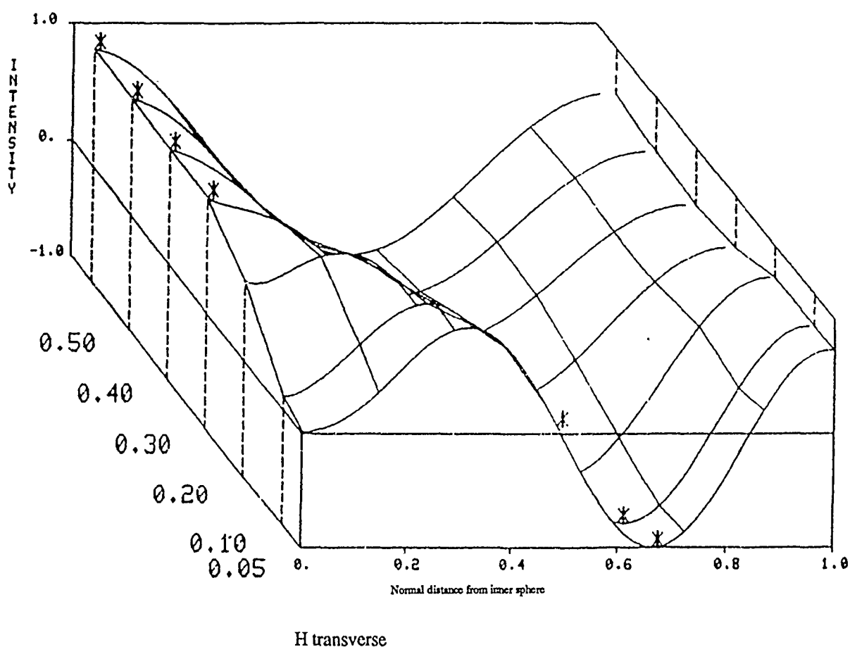
Figure 29. Distribution of the normalized transverse magnetic field component in the concentric spherical cavity as a function of the inner to outer conductor radii, R = b/a , for the TE 42 mode. Asterisk indicates peak value of field with d .
