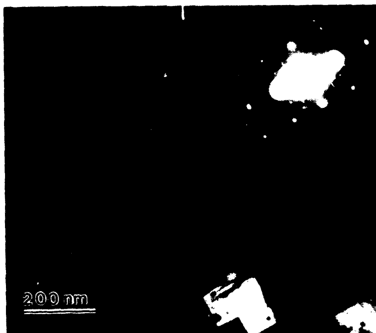
Figure 12B Dark-field TEM Micrograph of 6061 Aluminum Aged for 16 Hours at 473K.
