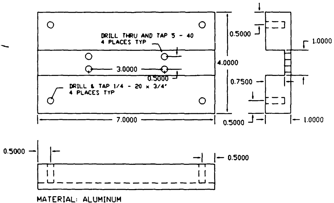
Figure A9 Base of new test rig. One required.
