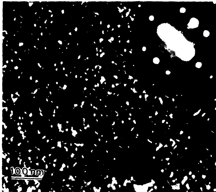
Figure 11B Dark-field TEM Micrograph of 6061 Aluminum Aged for 3000 Seconds at 473K.
