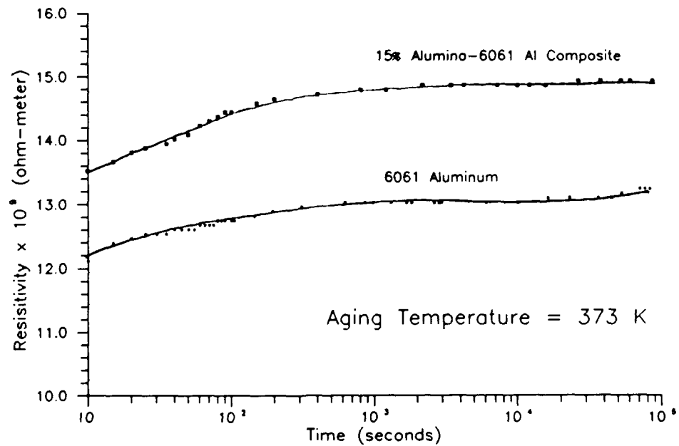
Figure 6 Resistivity of Alumina-6061 Aluminum Composite and 6061 Aluminum as a Function of Time at 373K.
