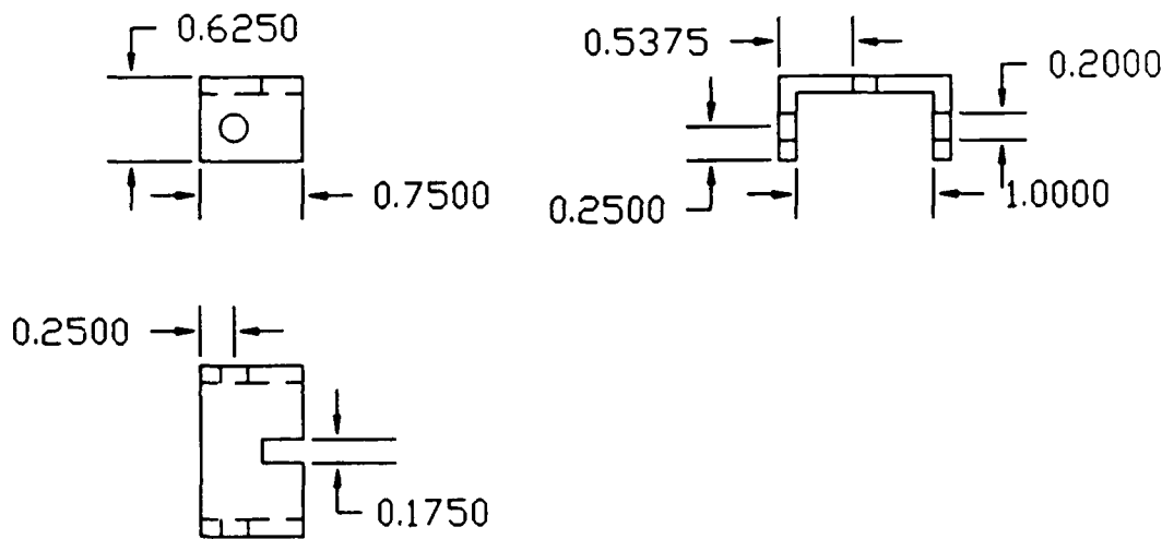
Figure A1 Guide to position probes on current test rig. Four required.
