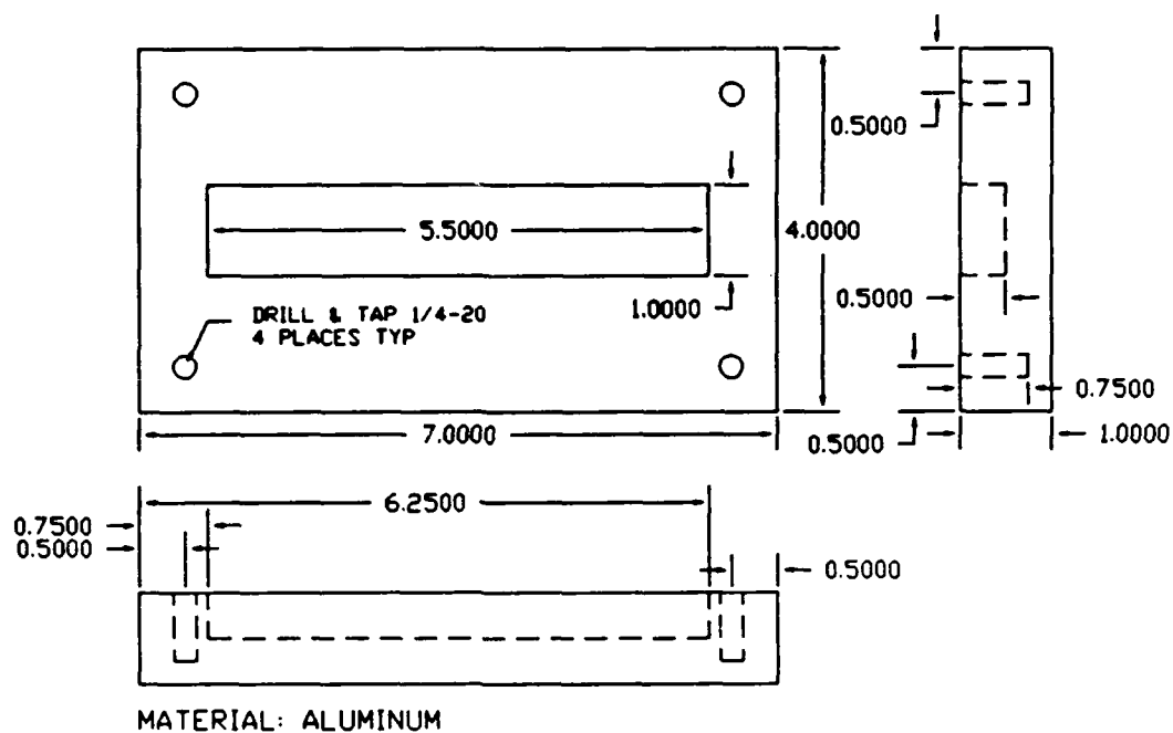
Figure A4 Base of present test rig. One required.
