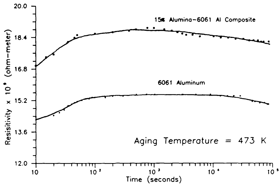
Figure 5 Resistivity of Alumina-6061 Aluminum Composite and 6061 Aluminum as a Function of Time at 473K.
