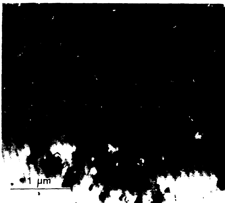
Figure 9B Dark-field TEM Micrograph of 6061 Aluminum Aged for 100 Seconds at 373K.
