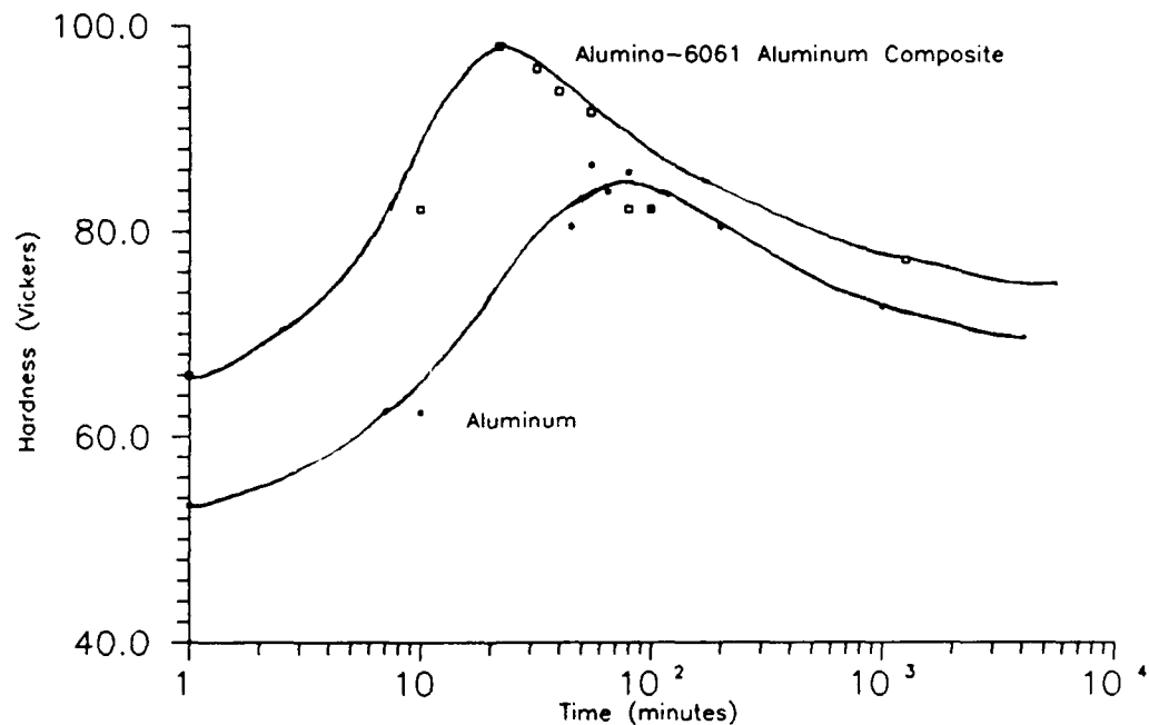
Figure 4: Results of Hardness Testing of 15 volume% reinforced \text{Al}_2\text{O}_3 compared to 6061 monolith.
