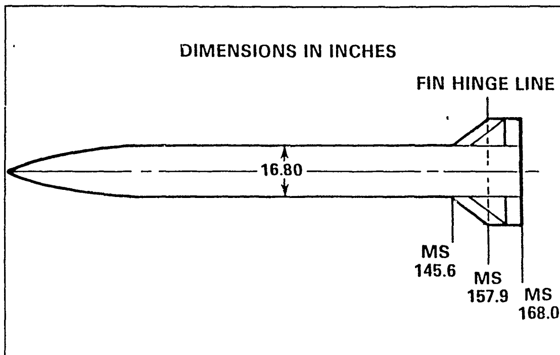
Figure 12. Air Slew Demonstrator [Ref. 54, p. 60]
