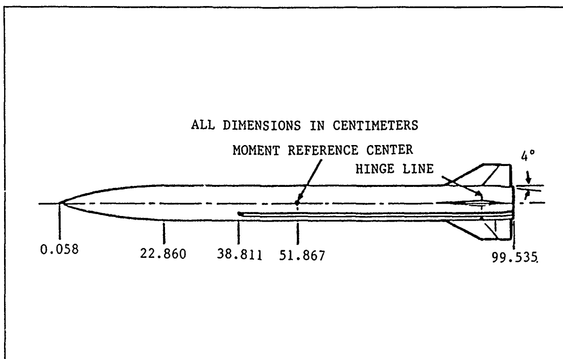
Figure 16. TMX-2774 (T-9 Tail) [Ref. 54, p. 42]
