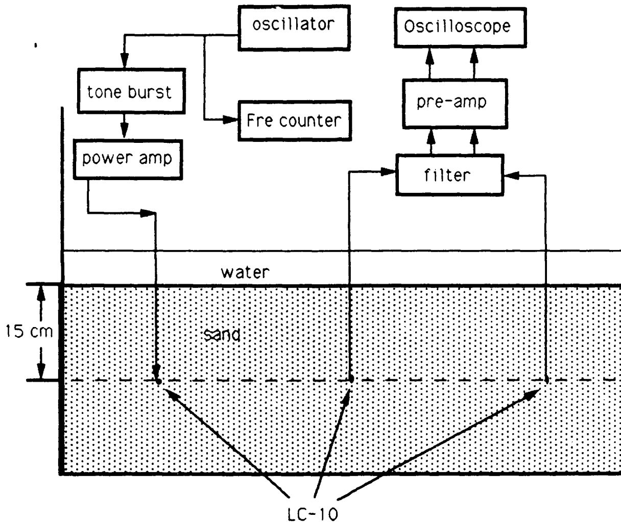
Figure 23 Measurement of the Speed of Sound in Water-Saturated Sand & Water.
