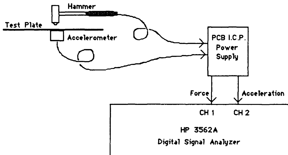
Figure 10. Plate Set Up for Impedance.
