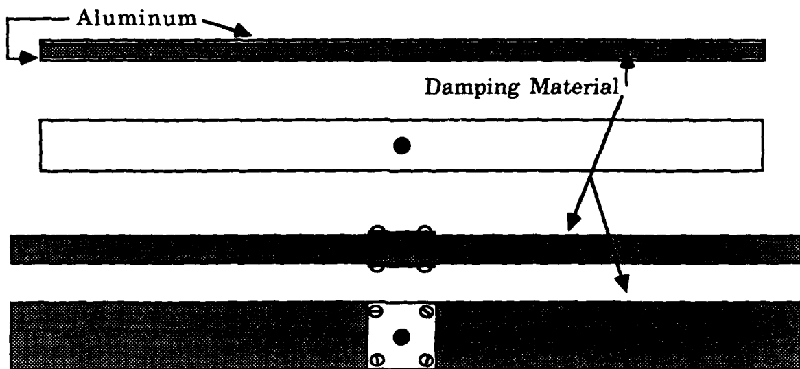
Figure 2. Constrained Layer and Single Layer Beams.
