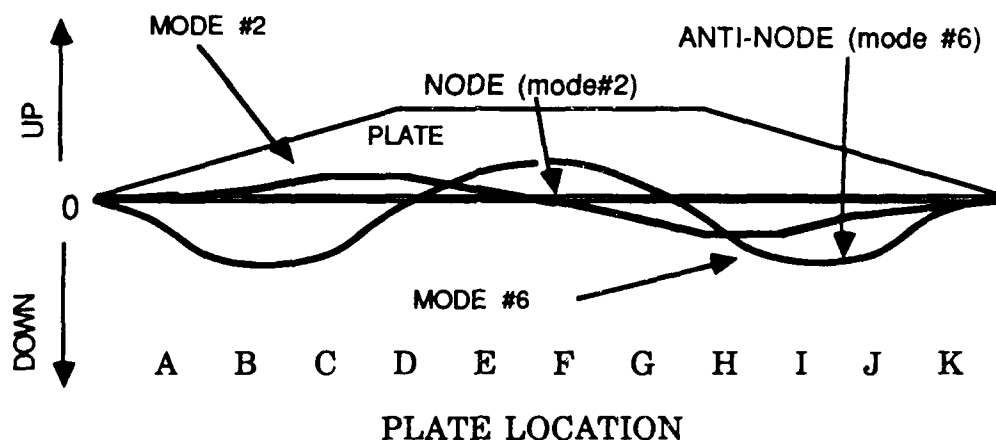
Figure 3. Exaggerated Relative Deflections across Section 6 of the Plate (not to scale).
