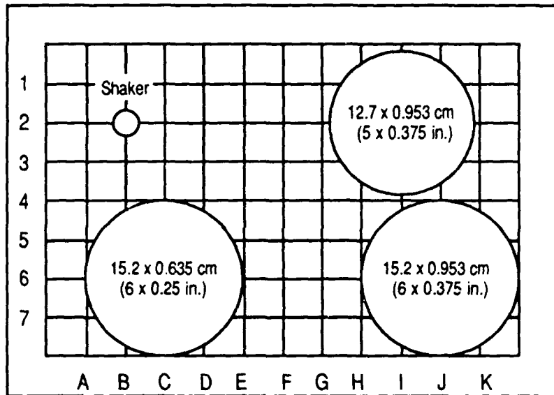
Figure 30. Waveguide Absorbers Mounted on Test Plate.
