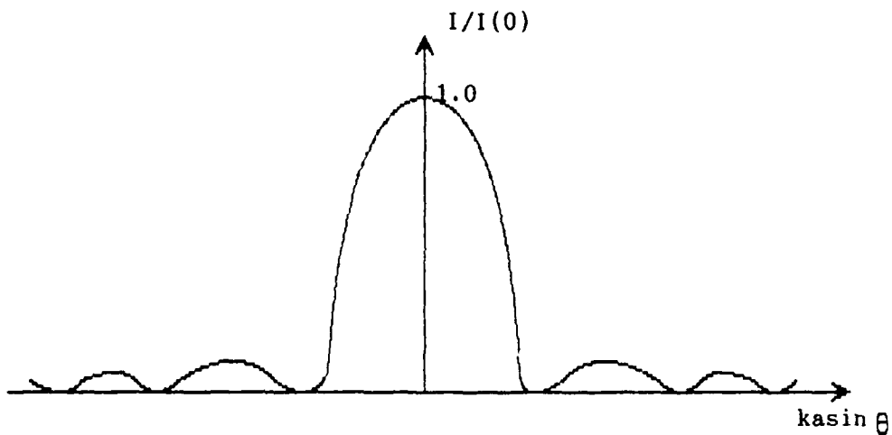
[Fig. 2] Airy function for circular aperture diffraction pattern
