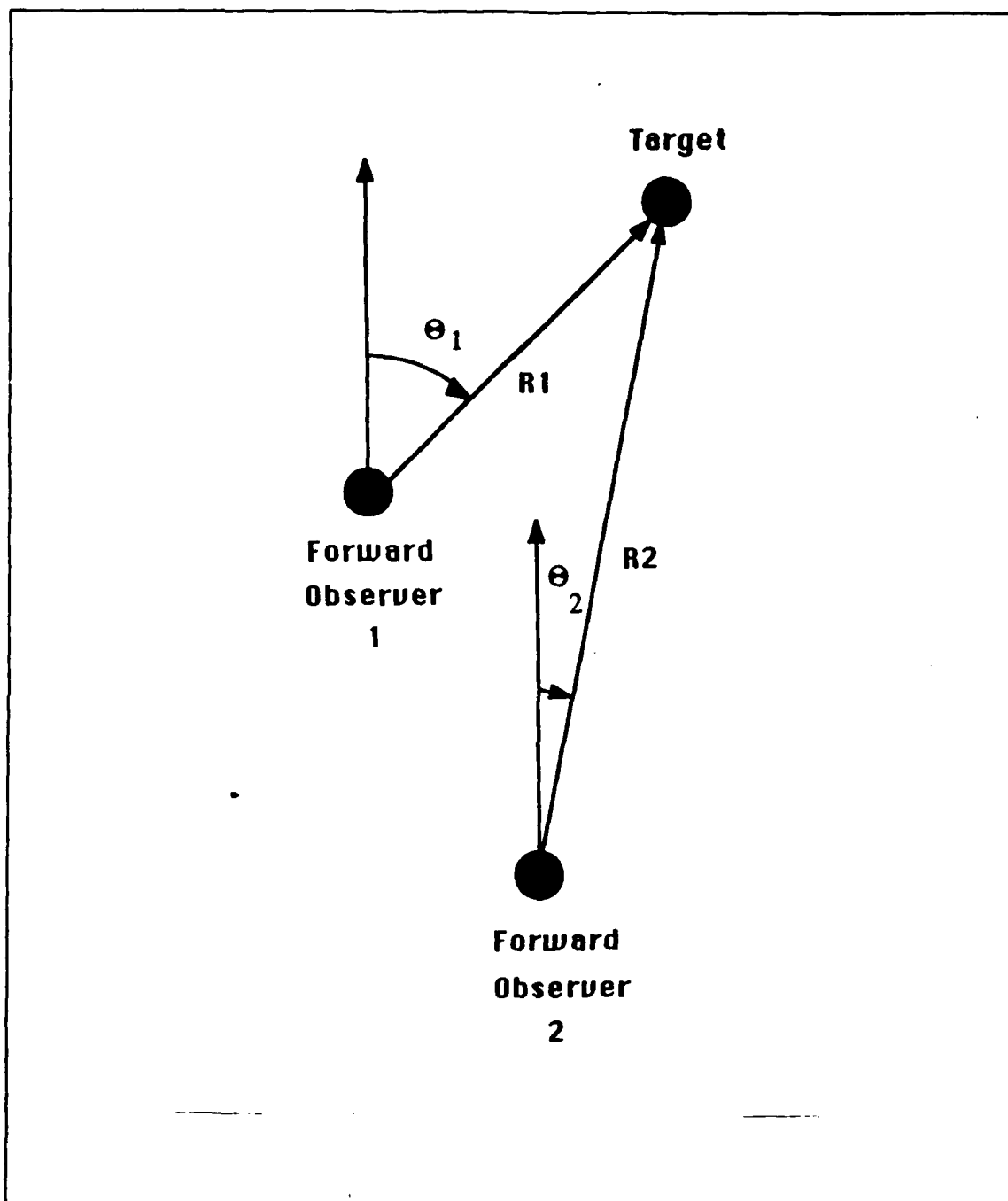
Figure 4. Bearings and Ranges Geometry: Measurement Inputs to the Kalman Filter are Restricted to Target Bearings and Target Ranges.
