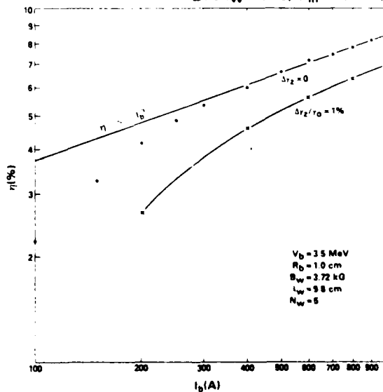
FIG. 14. Graph of the saturation efficiency of the TE_{01} mode vs beam current for \omega/ck_w = 11.3 .
